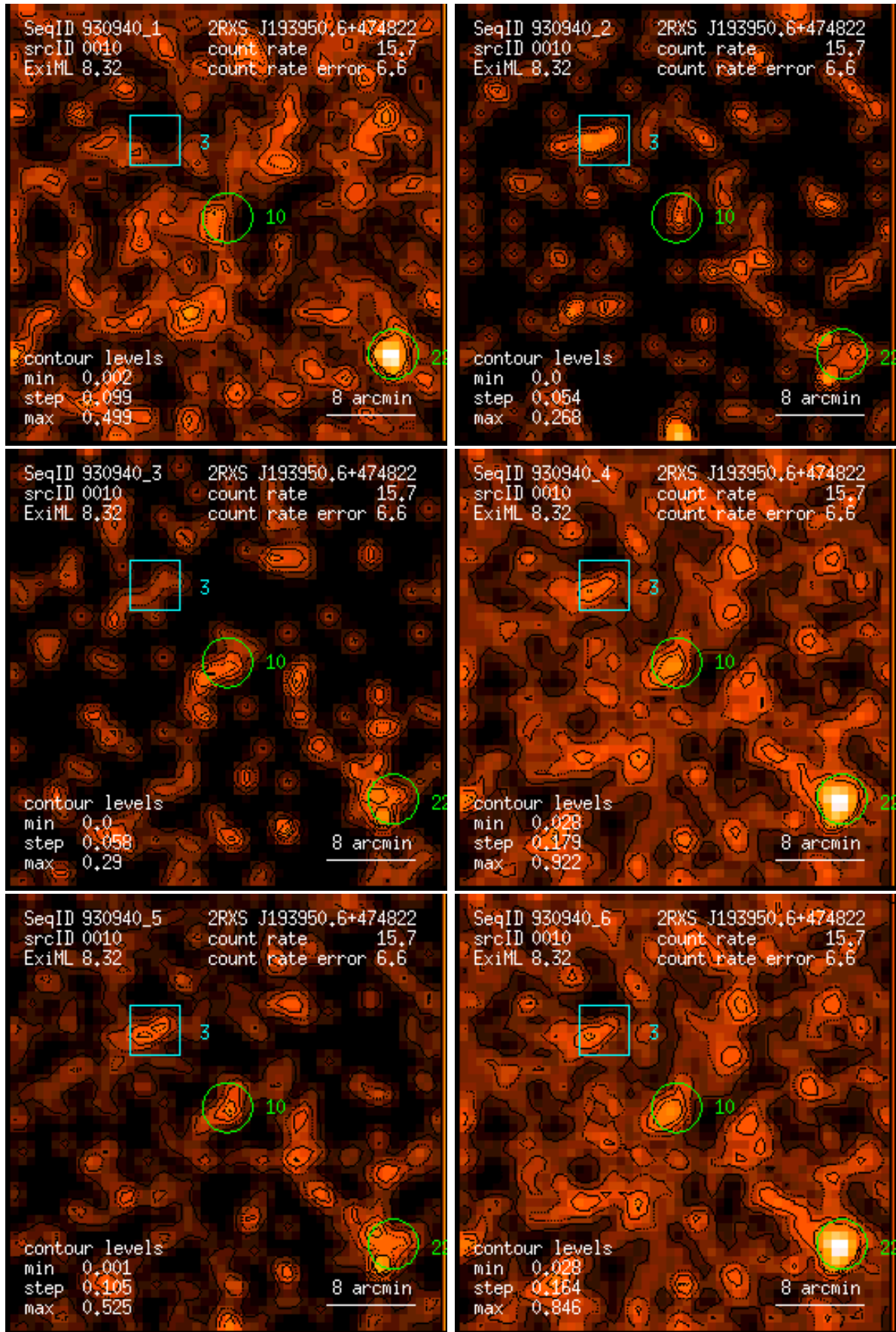
Figure 10: RASS 930940: detection 0010: band rate images, Gaussian filter: (1) PSPC channels 11 – 41, (2) 52 – 90, (3) 91 – 201, (4) 11 – 235, (5) 52 – 201, (6) 11 – 201. Broad band rates in counts/ks. Band rate contour levels in counts/ks/arcmin 2 .
