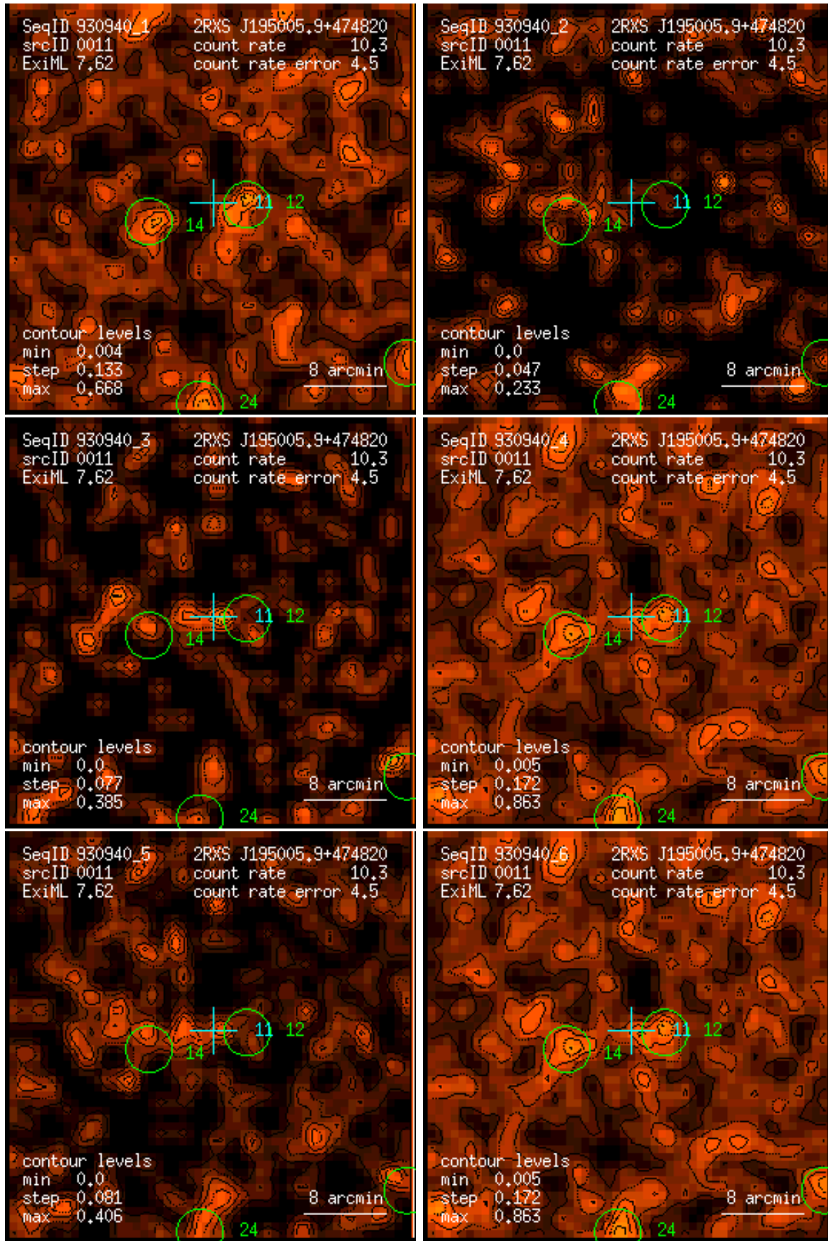
Figure 11: RASS 930940: detection 0011: band rate images, Gaussian filter: (1) PSPP channels 11 – 41, (2) 52 – 90, (3) 91 – 201, (4) 11 – 235, (5) 52 – 201, (6) 11 – 201. Broad band rates in counts/ks. Band rate contour levels in counts/ks/arcmin 2 .
