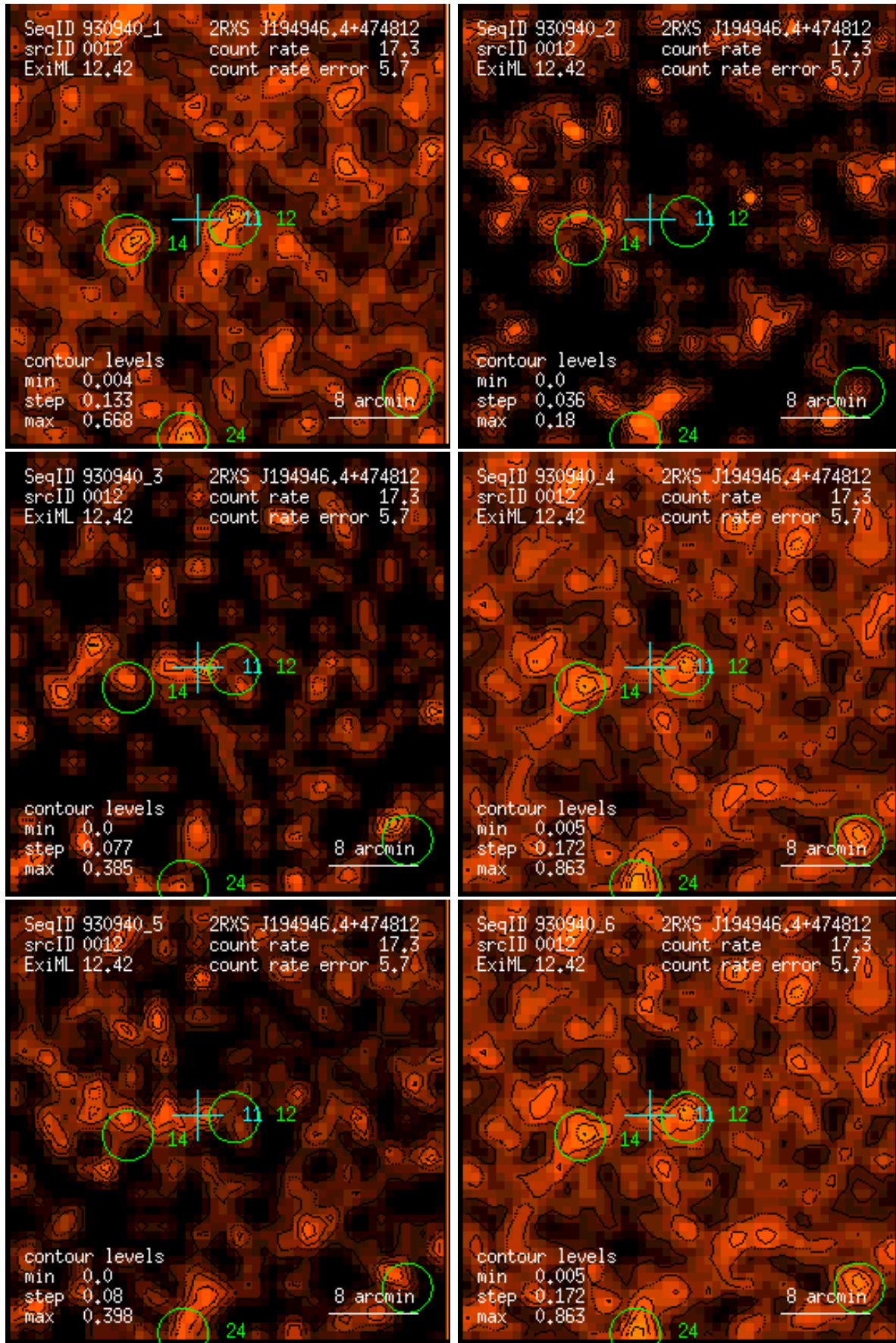
Figure 12: RASS 930940: detection 0012: band rate images, Gaussian filter: (1) PSPC channels 11 – 41, (2) 52 – 90, (3) 91 – 201, (4) 11 – 235, (5) 52 – 201, (6) 11 – 201. Broad band rates in counts/ks. Band rate contour levels in counts/ks/arcmin 2 .
