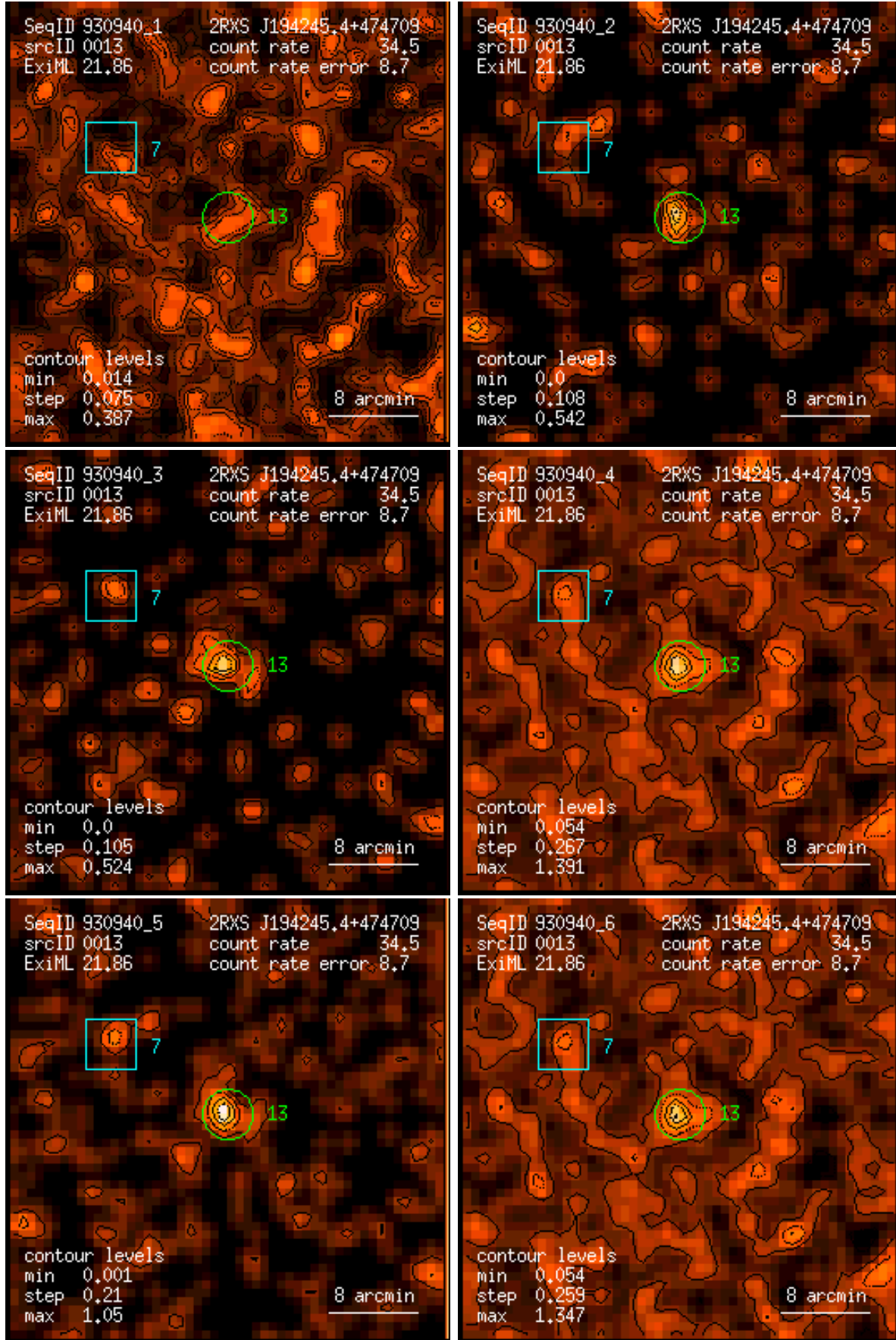
Figure 13: RASS 930940: detection 0013: band rate images, Gaussian filter: (1) PSPC channels 11 – 41, (2) 52 – 90, (3) 91 – 201, (4) 11 – 235, (5) 52 – 201, (6) 11 – 201. Broad band rates in counts/ks. Band rate contour levels in counts/ks/arcmin 2 .
