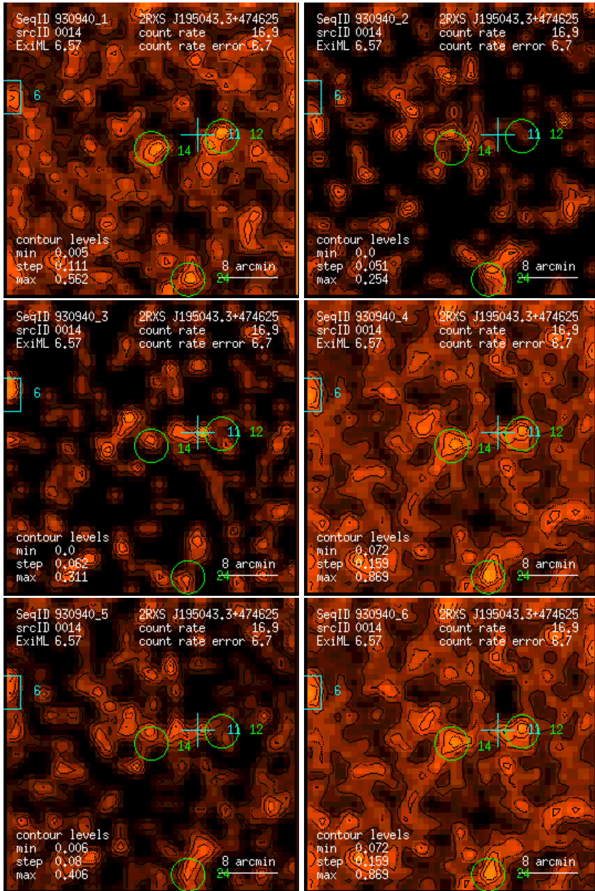
Figure 14: RASS 930940: detection 0014: band rate images, Gaussian filter: (1) PSPC channels 11 – 41, (2) 52 – 90, (3) 91 – 201, (4) 11 – 235, (5) 52 – 201, (6) 11 – 201. Broad band rates in counts/ks. Band rate contour levels in counts/ks/arcmin 2 .
