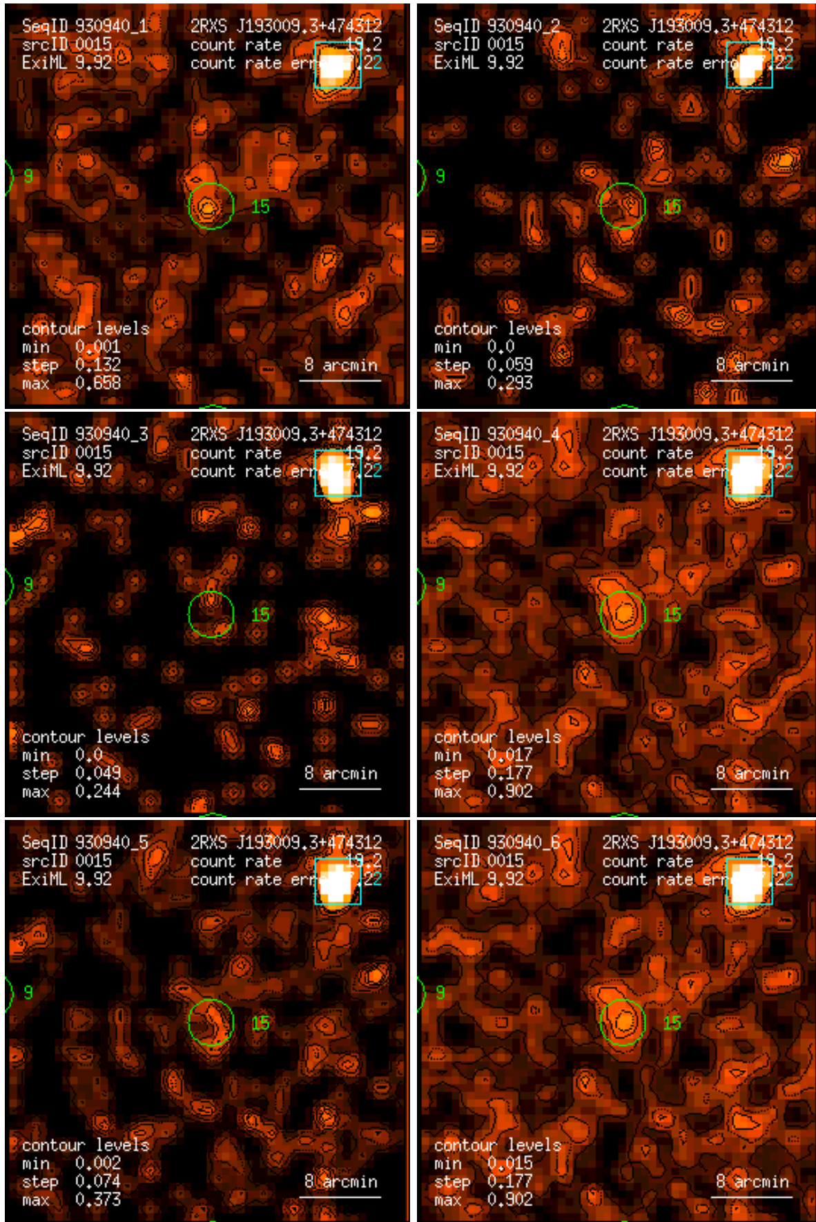
Figure 15: RASS 930940: detection 0015: band rate images, Gaussian filter: (1) PSPC channels 11 – 41, (2) 52 – 90, (3) 91 – 201, (4) 11 – 235, (5) 52 – 201, (6) 11 – 201. Broad band rates in counts/ks. Band rate contour levels in counts/ks/arcmin 2 .
