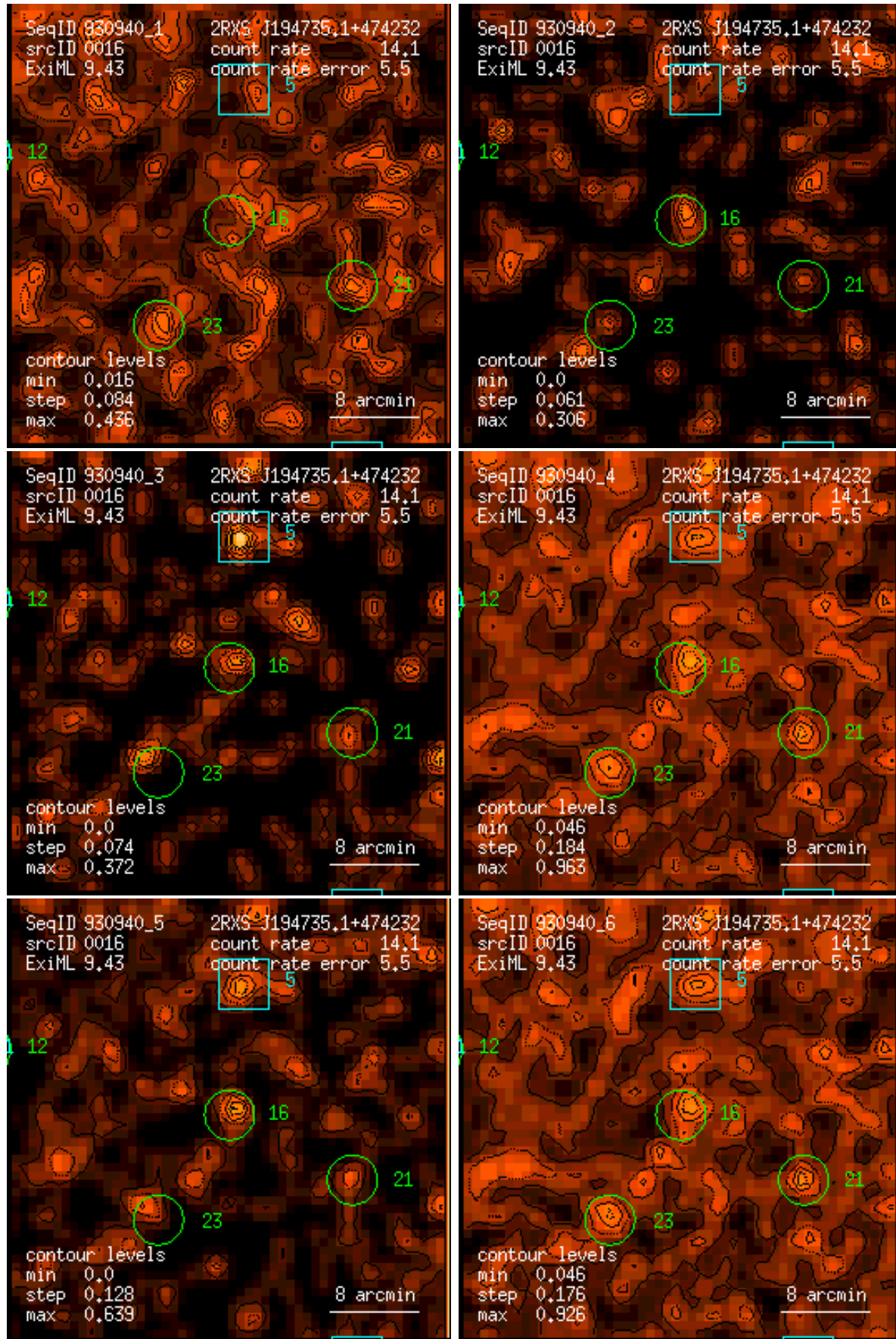
Figure 16: RASS 930940: detection 0016: band rate images, Gaussian filter: (1) PSPC channels 11 – 41, (2) 52 – 90, (3) 91 – 201, (4) 11 – 235, (5) 52 – 201, (6) 11 – 201. Broad band rates in counts/ks. Band rate contour levels in counts/ks/arcmin 2 .
