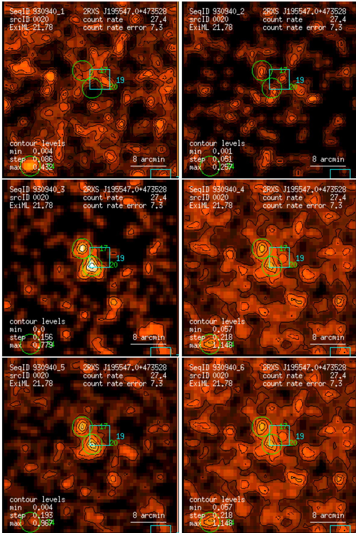
Figure 20: RASS 930940: detection 0020: band rate images, Gaussian filter: (1) PSPC channels 11 – 41, (2) 52 – 90, (3) 91 – 201, (4) 11 – 235, (5) 52 – 201, (6) 11 – 201. Broad band rates in counts/ks. Band rate contour levels in counts/ks/arcmin 2 .
