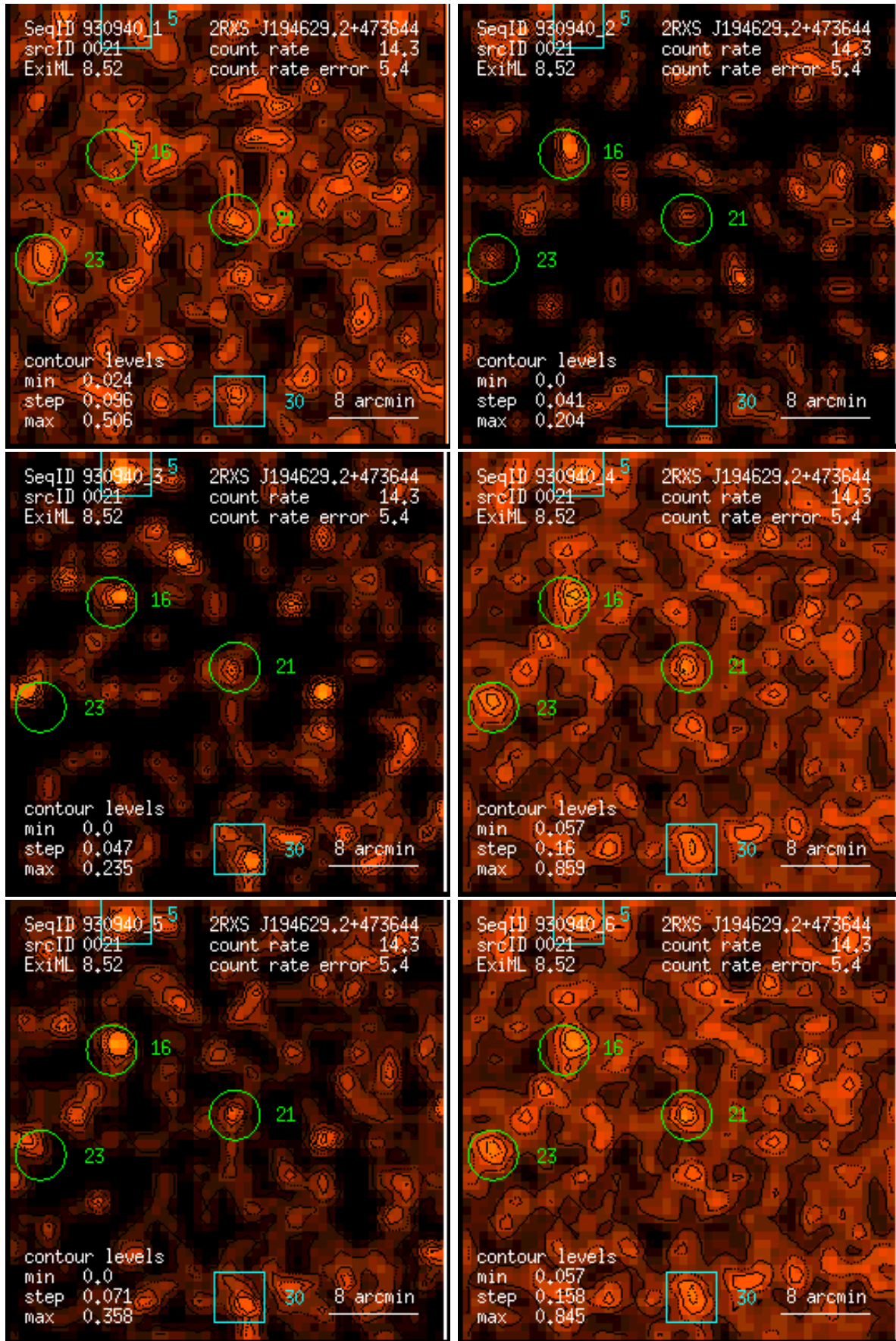
Figure 21: RASS 930940: detection 0021: band rate images, Gaussian filter: (1) PSPC channels 11 – 41, (2) 52 – 90, (3) 91 – 201, (4) 11 – 235, (5) 52 – 201, (6) 11 – 201. Broad band rates in counts/ks. Band rate contour levels in counts/ks/arcmin 2 .
