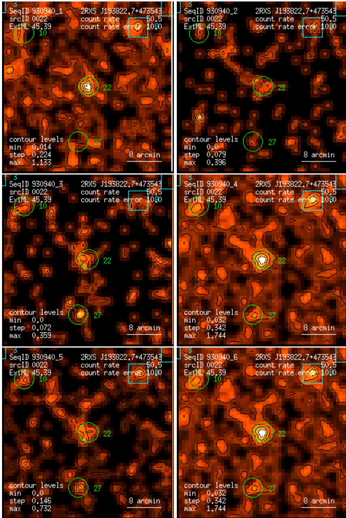
Figure 22: RASS 930940: detection 0022: band rate images, Gaussian filter: (1) PSPC channels 11 – 41, (2) 52 – 90, (3) 91 – 201, (4) 11 – 235, (5) 52 – 201, (6) 11 – 201. Broad band rates in counts/ks. Band rate contour levels in counts/ks/arcmin 2 .
