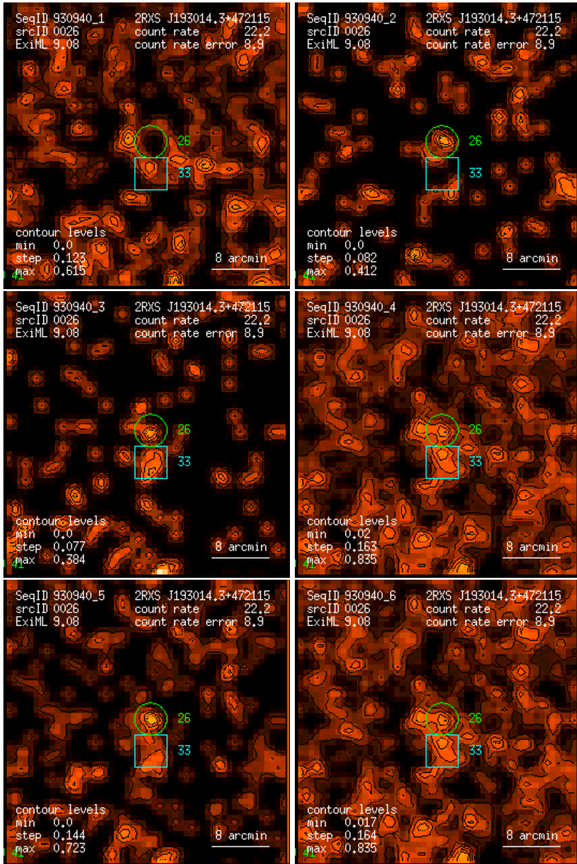
Figure 26: RASS 930940: detection 0026: band rate images, Gaussian filter: (1) PSPC channels 11 – 41, (2) 52 – 90, (3) 91 – 201, (4) 11 – 235, (5) 52 – 201, (6) 11 – 201. Broad band rates in counts/ks. Band rate contour levels in counts/ks/arcmin 2 .
