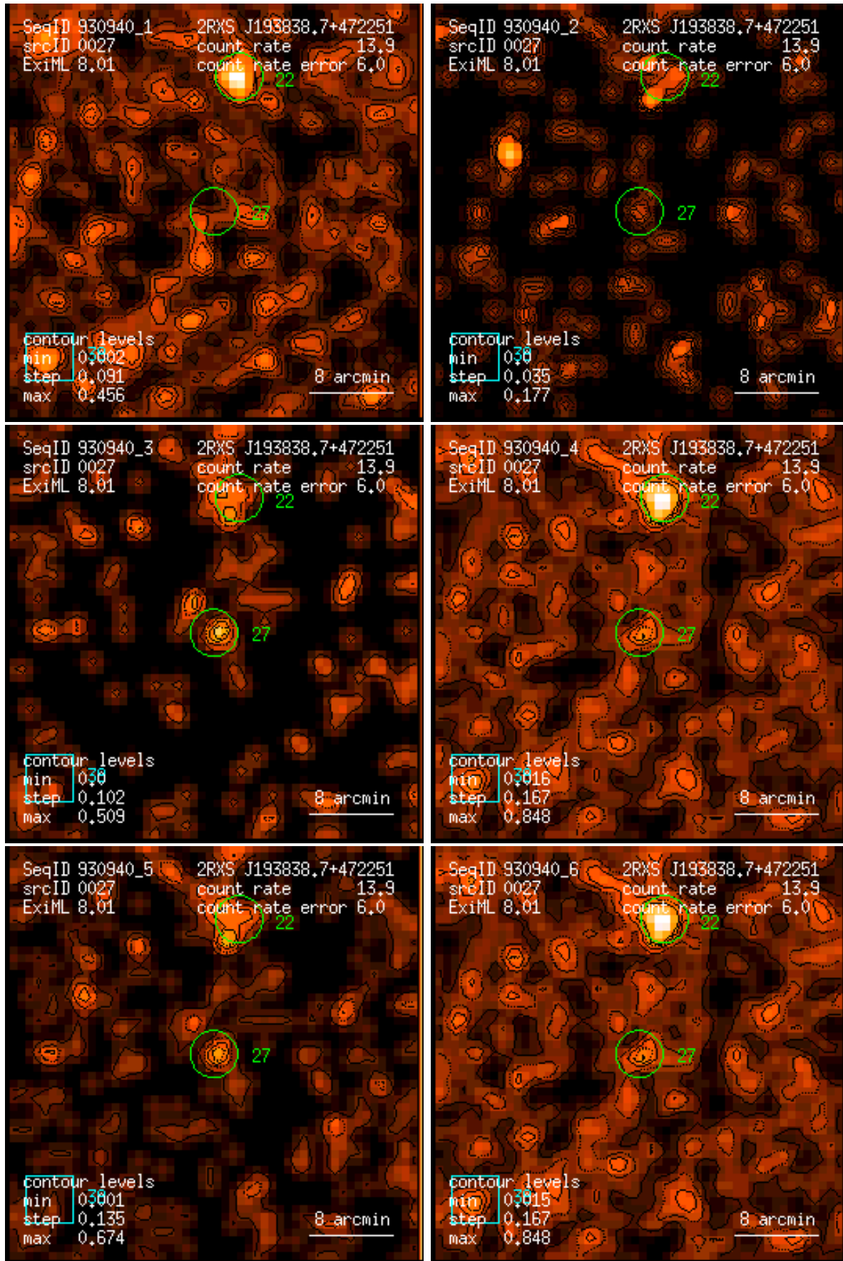
Figure 27: RASS 930940: detection 0027: band rate images, Gaussian filter: (1) PSPC channels 11 – 41, (2) 52 – 90, (3) 91 – 201, (4) 11 – 235, (5) 52 – 201, (6) 11 – 201. Broad band rates in counts/ks. Band rate contour levels in counts/ks/arcmin 2 .
