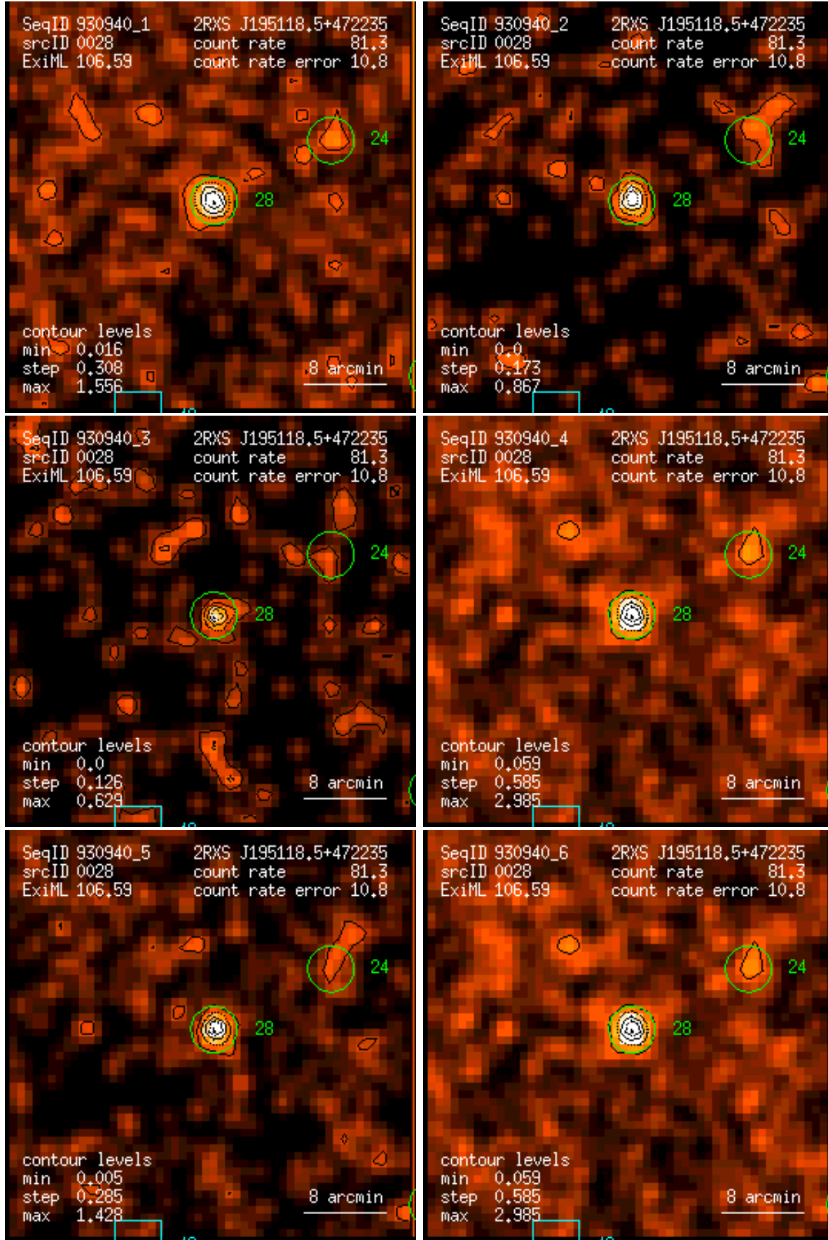
Figure 28: RASS 930940: detection 0028: band rate images, Gaussian filter: (1) PSPC channels 11 – 41, (2) 52 – 90, (3) 91 – 201, (4) 11 – 235, (5) 52 – 201, (6) 11 – 201. Broad band rates in counts/ks. Band rate contour levels in counts/ks/arcmin 2 .
