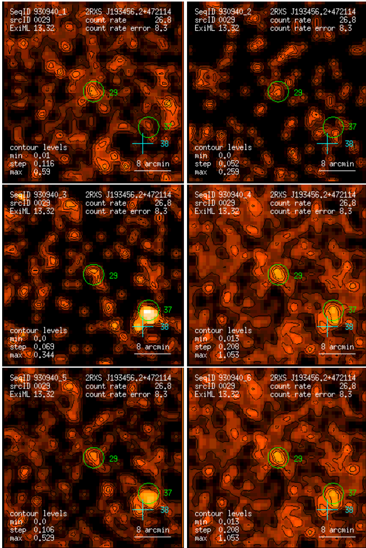
Figure 29: RASS 930940: detection 0029: band rate images, Gaussian filter: (1) PSPC channels 11 – 41, (2) 52 – 90, (3) 91 – 201, (4) 11 – 235, (5) 52 – 201, (6) 11 – 201. Broad band rates in counts/ks. Band rate contour levels in counts/ks/arcmin 2 .
