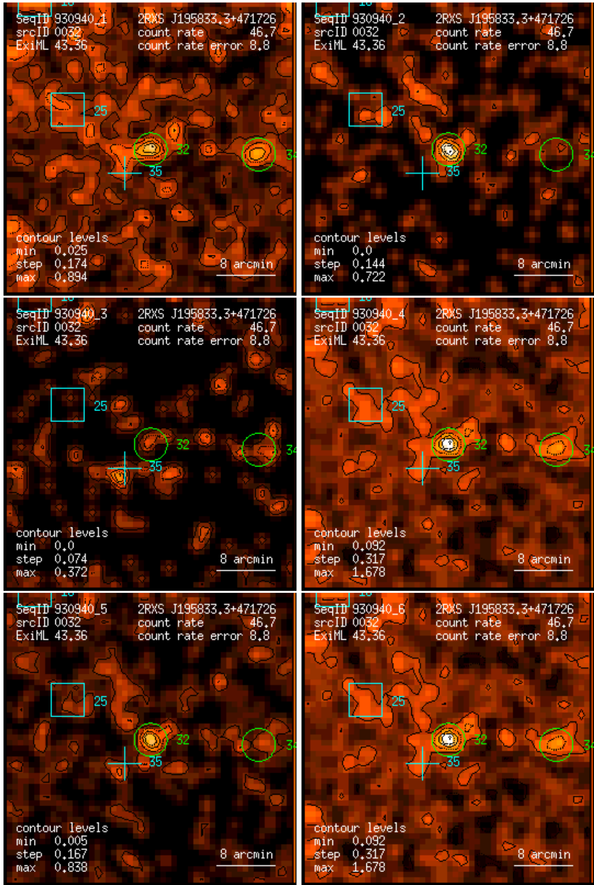
Figure 32: RASS 930940: detection 0032: band rate images, Gaussian filter: (1) PSPC channels 11 – 41, (2) 52 – 90, (3) 91 – 201, (4) 11 – 235, (5) 52 – 201, (6) 11 – 201. Broad band rates in counts/ks. Band rate contour levels in counts/ks/arcmin 2 .
