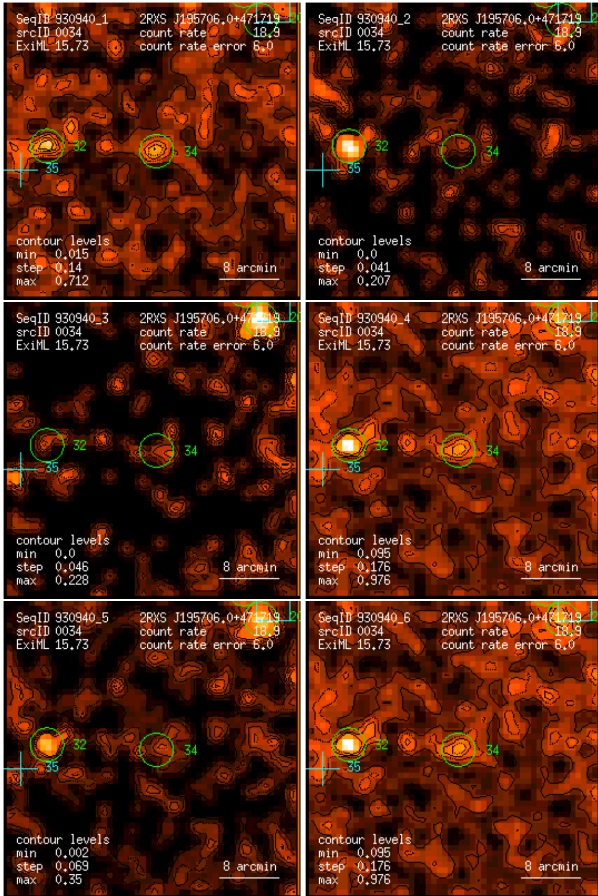
Figure 34: RASS 930940: detection 0034: band rate images, Gaussian filter: (1) PSPC channels 11 – 41, (2) 52 – 90, (3) 91 – 201, (4) 11 – 235, (5) 52 – 201, (6) 11 – 201. Broad band rates in counts/ks. Band rate contour levels in counts/ks/arcmin 2 .
