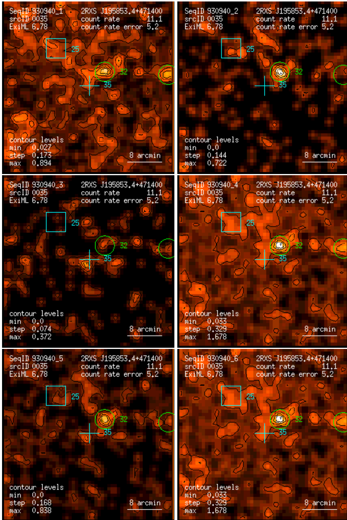
Figure 35: RASS 930940: detection 0035: band rate images, Gaussian filter: (1) PSPC channels 11 – 41, (2) 52 – 90, (3) 91 – 201, (4) 11 – 235, (5) 52 – 201, (6) 11 – 201. Broad band rates in counts/ks. Band rate contour levels in counts/ks/arcmin 2 .
