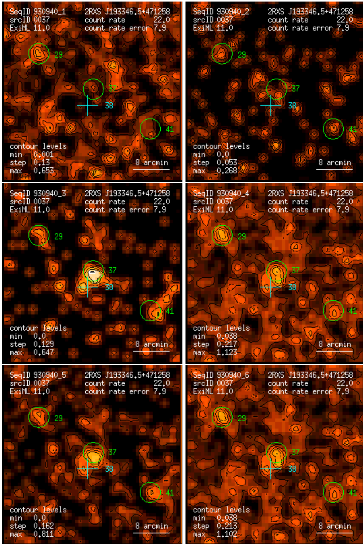
Figure 37: RASS 930940: detection 0037: band rate images, Gaussian filter: (1) PSPC channels 11 – 41, (2) 52 – 90, (3) 91 – 201, (4) 11 – 235, (5) 52 – 201, (6) 11 – 201. Broad band rates in counts/ks. Band rate contour levels in counts/ks/arcmin 2 .
