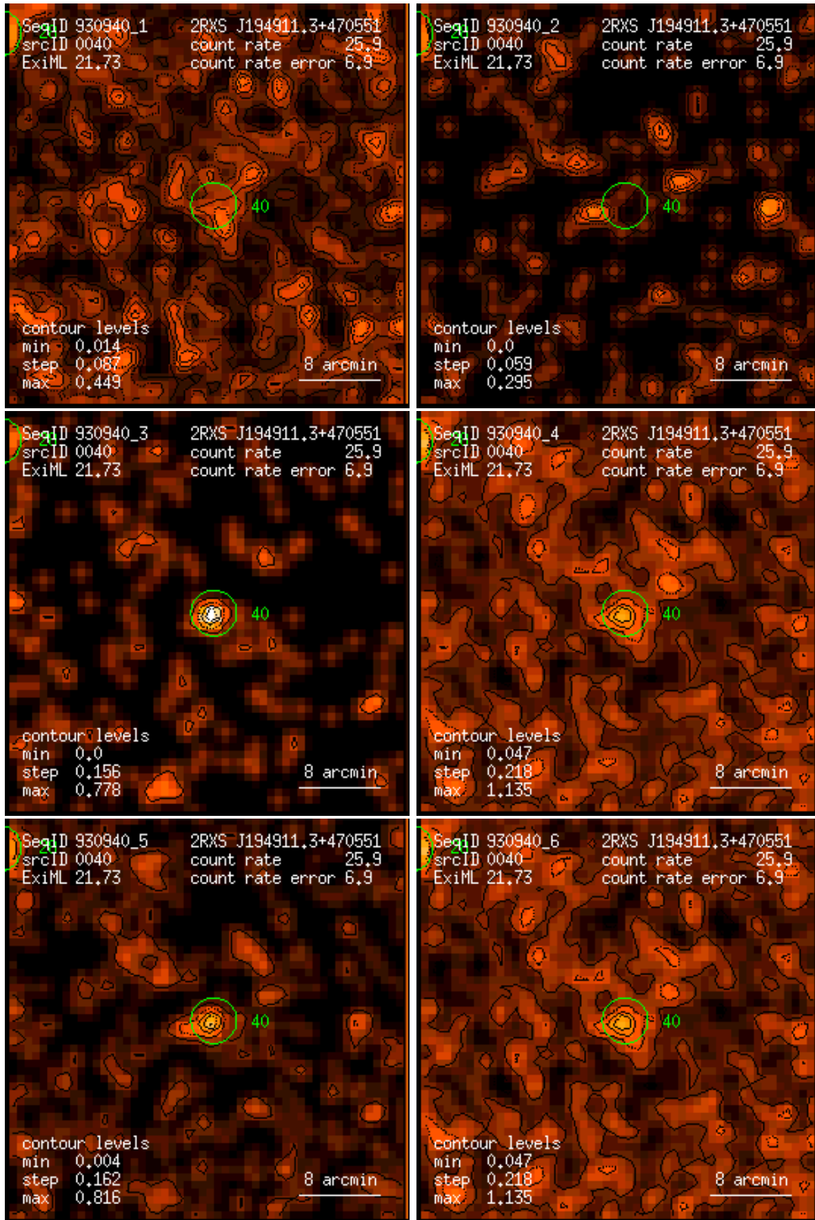
Figure 40: RASS 930940: detection 0040: band rate images, Gaussian filter: (1) PSPC channels 11 – 41, (2) 52 – 90, (3) 91 – 201, (4) 11 – 235, (5) 52 – 201, (6) 11 – 201. Broad band rates in counts/ks. Band rate contour levels in counts/ks/arcmin 2 .
