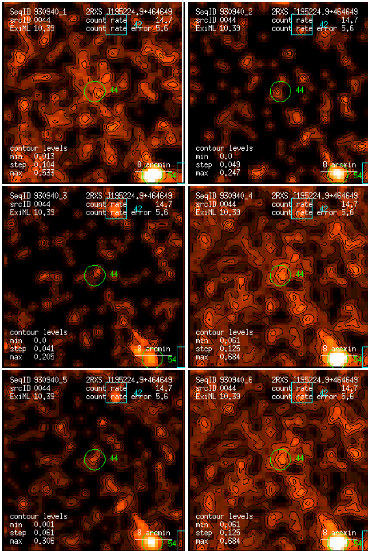
Figure 44: RASS 930940: detection 0044: band rate images, Gaussian filter: (1) PSPC channels 11 – 41, (2) 52 – 90, (3) 91 – 201, (4) 11 – 235, (5) 52 – 201, (6) 11 – 201. Broad band rates in counts/ks. Band rate contour levels in counts/ks/arcmin 2 .
