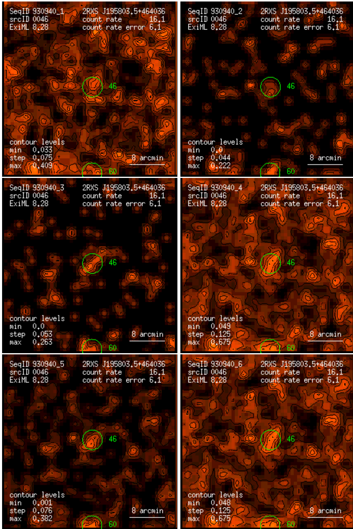
Figure 46: RASS 930940: detection 0046: band rate images, Gaussian filter: (1) PSPC channels 11 – 41, (2) 52 – 90, (3) 91 – 201, (4) 11 – 235, (5) 52 – 201, (6) 11 – 201. Broad band rates in counts/ks. Band rate contour levels in counts/ks/arcmin 2 .
