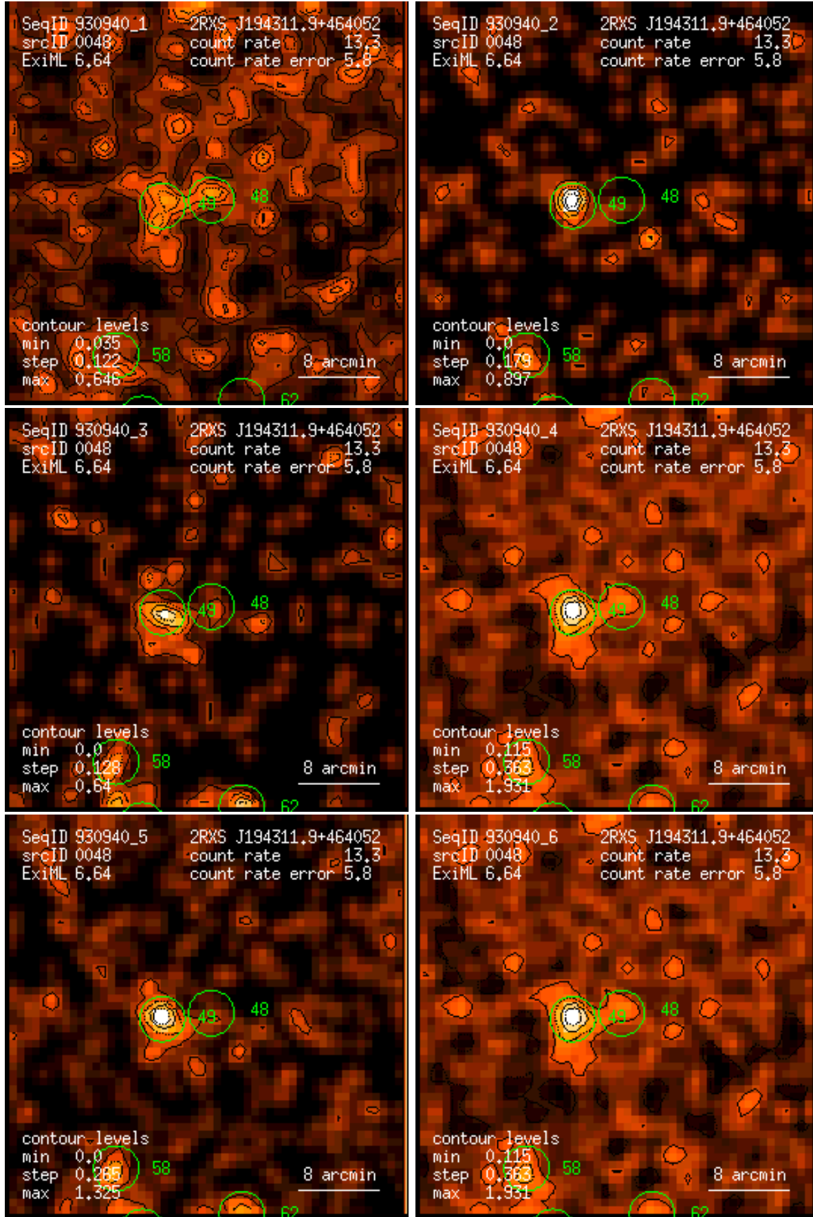
Figure 48: RASS 930940: detection 0048: band rate images, Gaussian filter: (1) PSPC channels 11 – 41, (2) 52 – 90, (3) 91 – 201, (4) 11 – 235, (5) 52 – 201, (6) 11 – 201. Broad band rates in counts/ks. Band rate contour levels in counts/ks/arcmin 2 .
