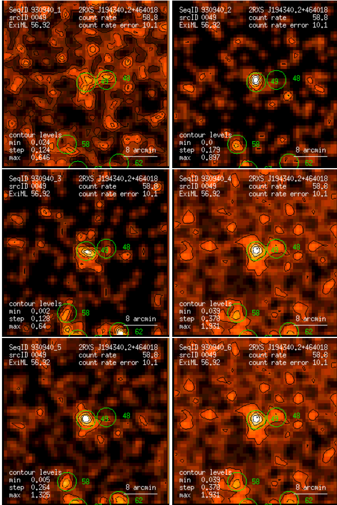
Figure 49: RASS 930940: detection 0049: band rate images, Gaussian filter: (1) PSPC channels 11 – 41, (2) 52 – 90, (3) 91 – 201, (4) 11 – 235, (5) 52 – 201, (6) 11 – 201. Broad band rates in counts/ks. Band rate contour levels in counts/ks/arcmin 2 .
