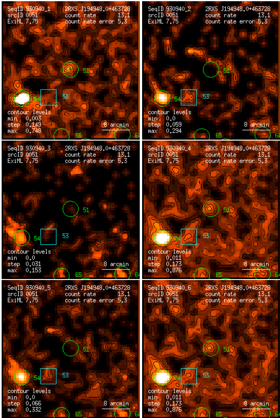
Figure 51: RASS 930940: detection 0051: band rate images, Gaussian filter: (1) PSPC channels 11 – 41, (2) 52 – 90, (3) 91 – 201, (4) 11 – 235, (5) 52 – 201, (6) 11 – 201. Broad band rates in counts/ks. Band rate contour levels in counts/ks/arcmin 2 .
