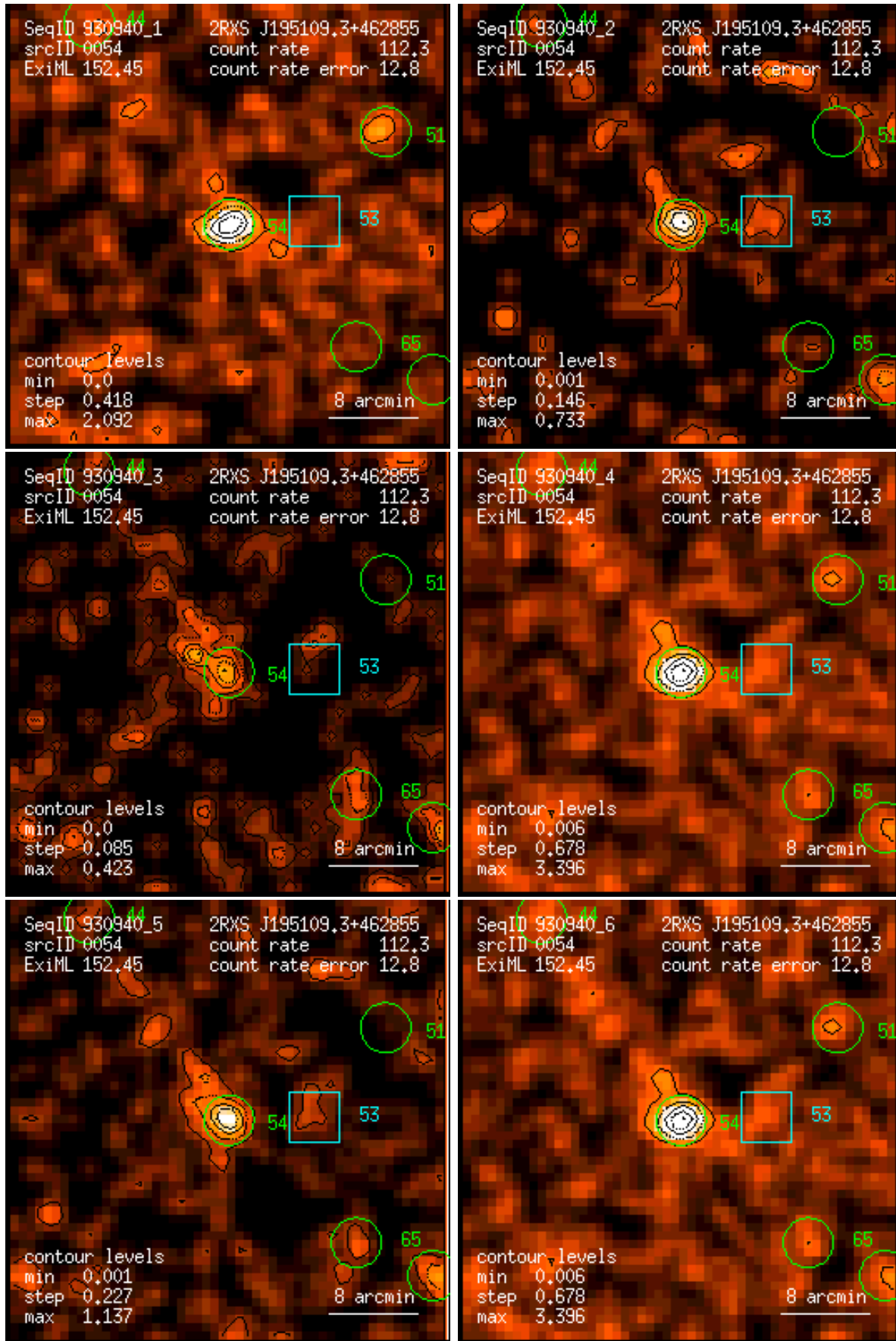
Figure 54: RASS 930940: detection 0054: band rate images, Gaussian filter: (1) PSPC channels 11 – 41, (2) 52 – 90, (3) 91 – 201, (4) 11 – 235, (5) 52 – 201, (6) 11 – 201. Broad band rates in counts/ks. Band rate contour levels in counts/ks/arcmin 2 .
