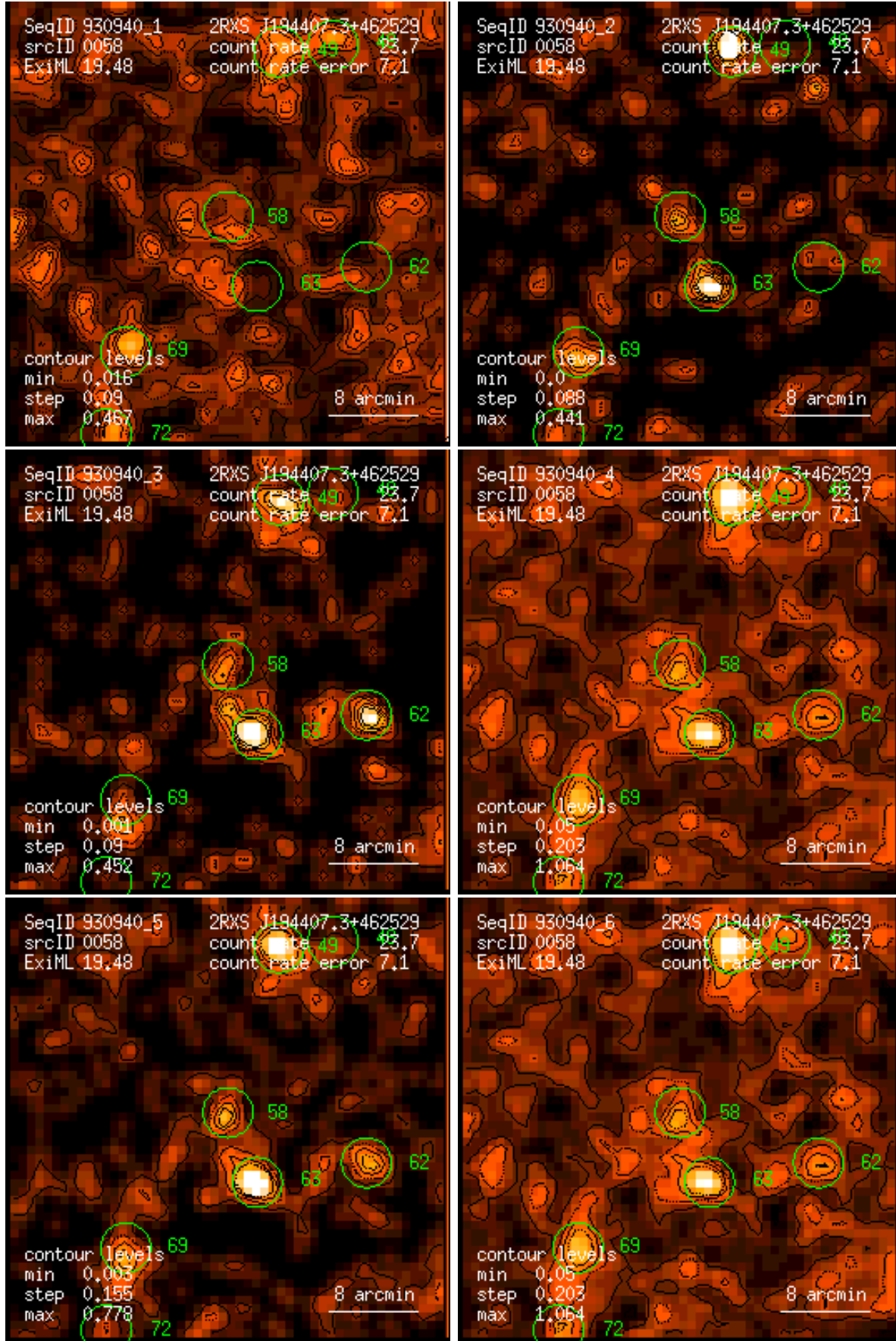
Figure 58: RASS 930940: detection 0058: band rate images, Gaussian filter: (1) PSPC channels 11 – 41, (2) 52 – 90, (3) 91 – 201, (4) 11 – 235, (5) 52 – 201, (6) 11 – 201. Broad band rates in counts/ks. Band rate contour levels in counts/ks/arcmin 2 .
