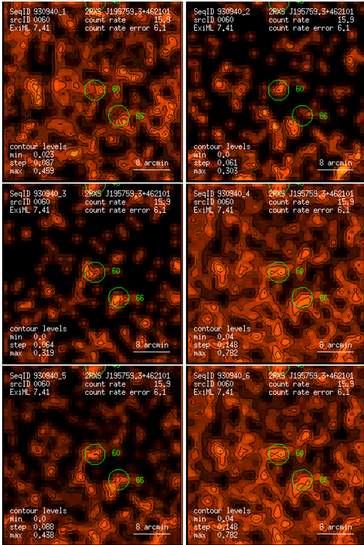
Figure 60: RASS 930940: detection 0060: band rate images, Gaussian filter: (1) PSPC channels 11 – 41, (2) 52 – 90, (3) 91 – 201, (4) 11 – 235, (5) 52 – 201, (6) 11 – 201. Broad band rates in counts/ks. Band rate contour levels in counts/ks/arcmin 2 .
