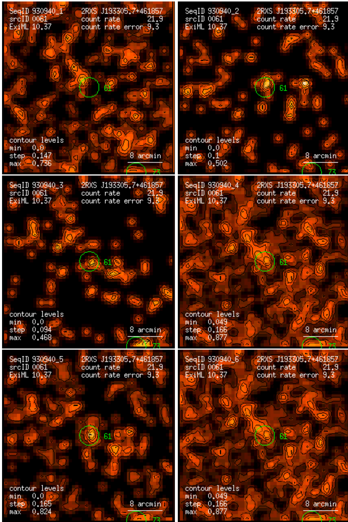
Figure 61: RASS 930940: detection 0061: band rate images, Gaussian filter: (1) PSPC channels 11 – 41, (2) 52 – 90, (3) 91 – 201, (4) 11 – 235, (5) 52 – 201, (6) 11 – 201. Broad band rates in counts/ks. Band rate contour levels in counts/ks/arcmin 2 .
