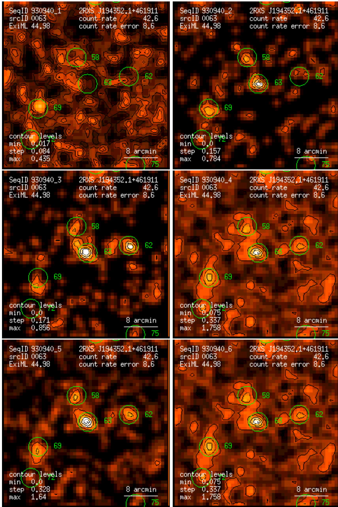
Figure 63: RASS 930940: detection 0063: band rate images, Gaussian filter: (1) PSPC channels 11 – 41, (2) 52 – 90, (3) 91 – 201, (4) 11 – 235, (5) 52 – 201, (6) 11 – 201. Broad band rates in counts/ks. Band rate contour levels in counts/ks/arcmin 2 .
