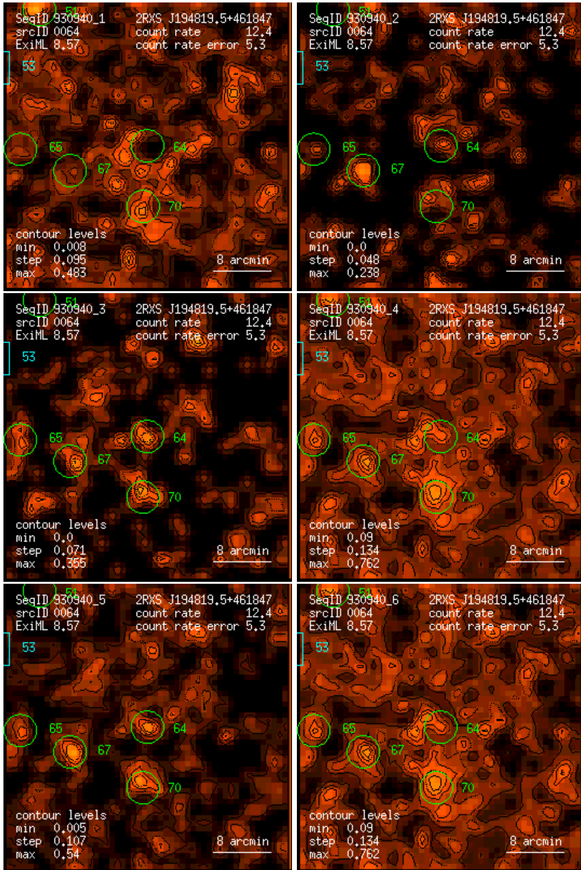
Figure 64: RASS 930940: detection 0064: band rate images, Gaussian filter: (1) PSPC channels 11 – 41, (2) 52 – 90, (3) 91 – 201, (4) 11 – 235, (5) 52 – 201, (6) 11 – 201. Broad band rates in counts/ks. Band rate contour levels in counts/ks/arcmin 2 .
