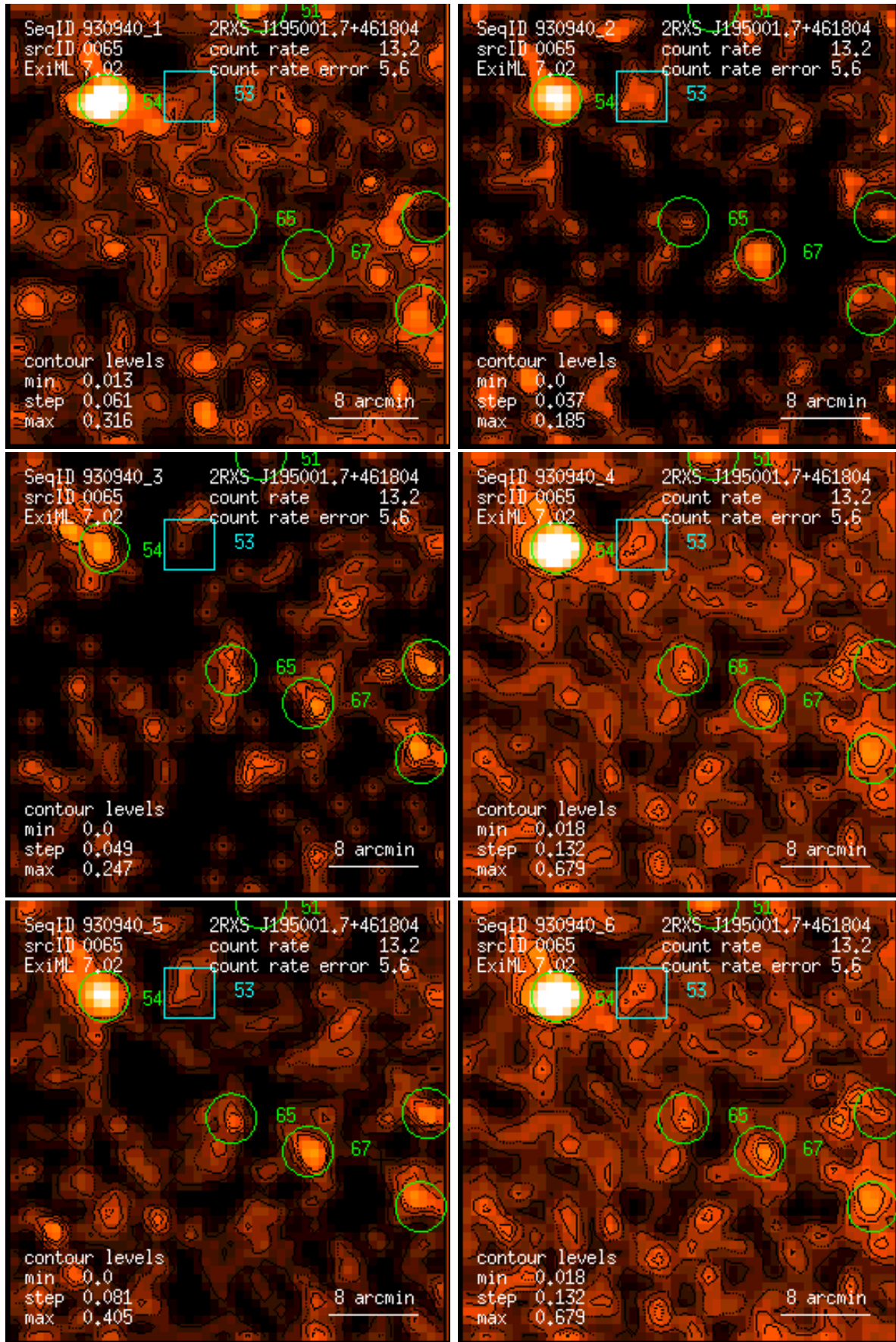
Figure 65: RASS 930940: detection 0065: band rate images, Gaussian filter: (1) PSPC channels 11 – 41, (2) 52 – 90, (3) 91 – 201, (4) 11 – 235, (5) 52 – 201, (6) 11 – 201. Broad band rates in counts/ks. Band rate contour levels in counts/ks/arcmin 2 .
