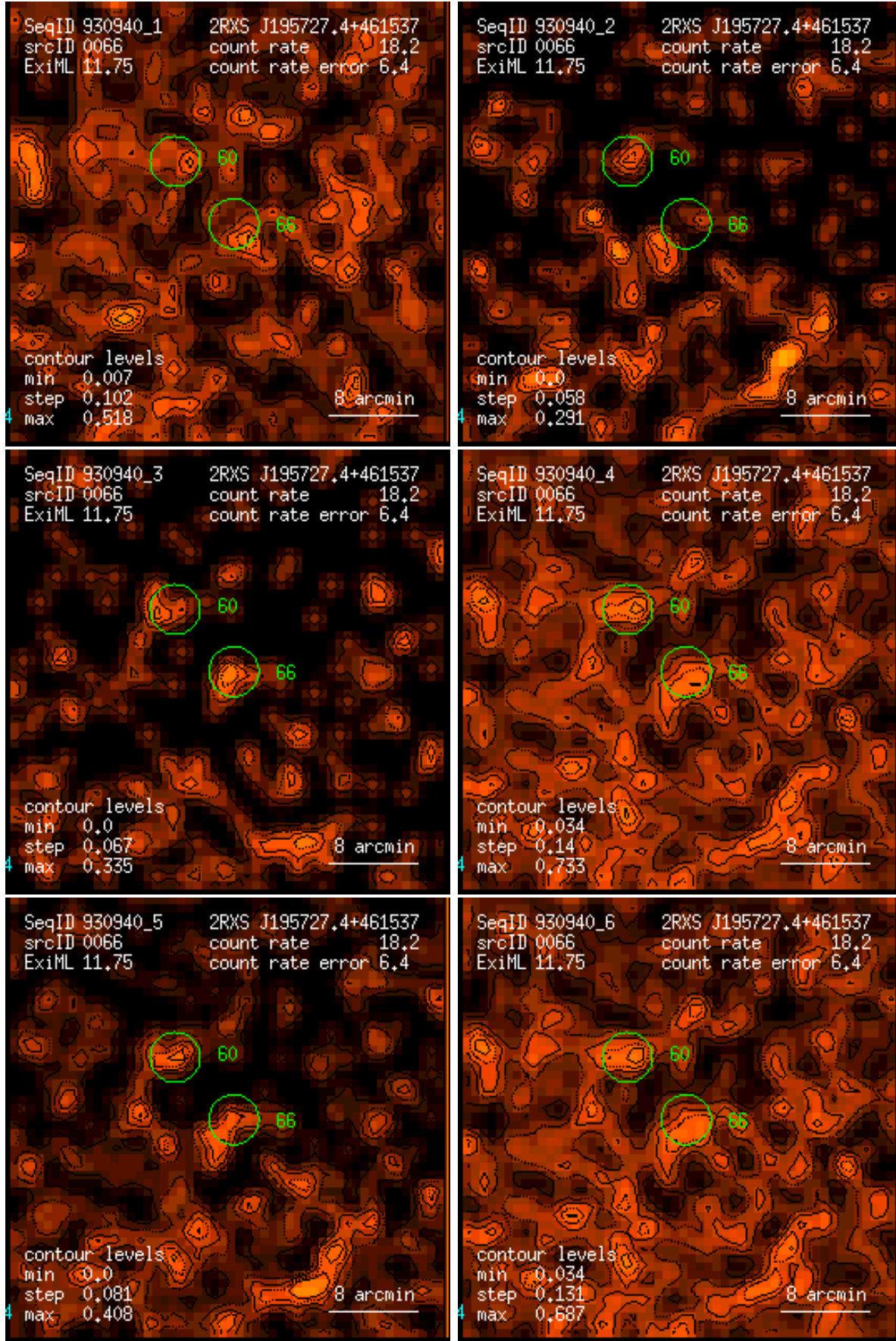
Figure 66: RASS 930940: detection 0066: band rate images, Gaussian filter: (1) PSPC channels 11 – 41, (2) 52 – 90, (3) 91 – 201, (4) 11 – 235, (5) 52 – 201, (6) 11 – 201. Broad band rates in counts/ks. Band rate contour levels in counts/ks/arcmin 2 .
