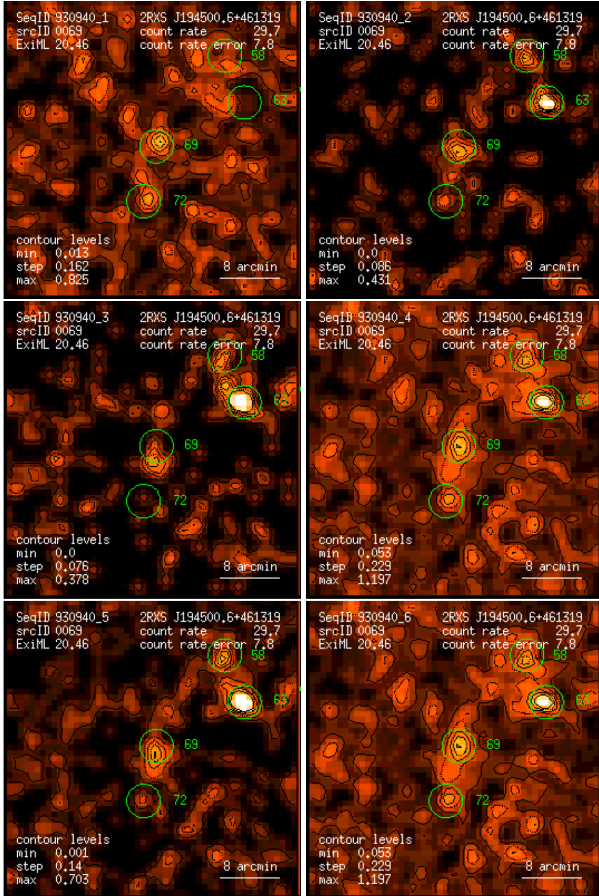
Figure 69: RASS 930940: detection 0069: band rate images, Gaussian filter: (1) PSPC channels 11 – 41, (2) 52 – 90, (3) 91 – 201, (4) 11 – 235, (5) 52 – 201, (6) 11 – 201. Broad band rates in counts/ks. Band rate contour levels in counts/ks/arcmin 2 .
