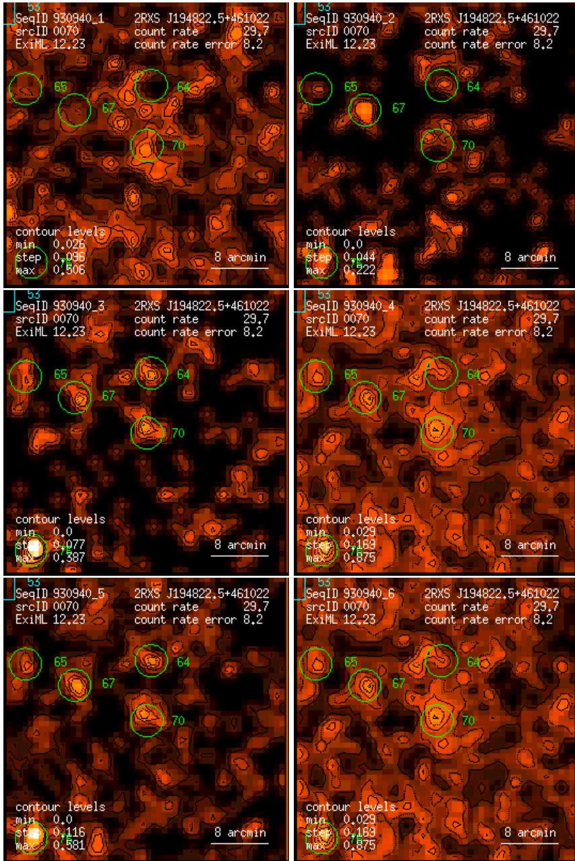
Figure 70: RASS 930940: detection 0070: band rate images, Gaussian filter: (1) PSPC channels 11 – 41, (2) 52 – 90, (3) 91 – 201, (4) 11 – 235, (5) 52 – 201, (6) 11 – 201. Broad band rates in counts/ks. Band rate contour levels in counts/ks/arcmin 2 .
