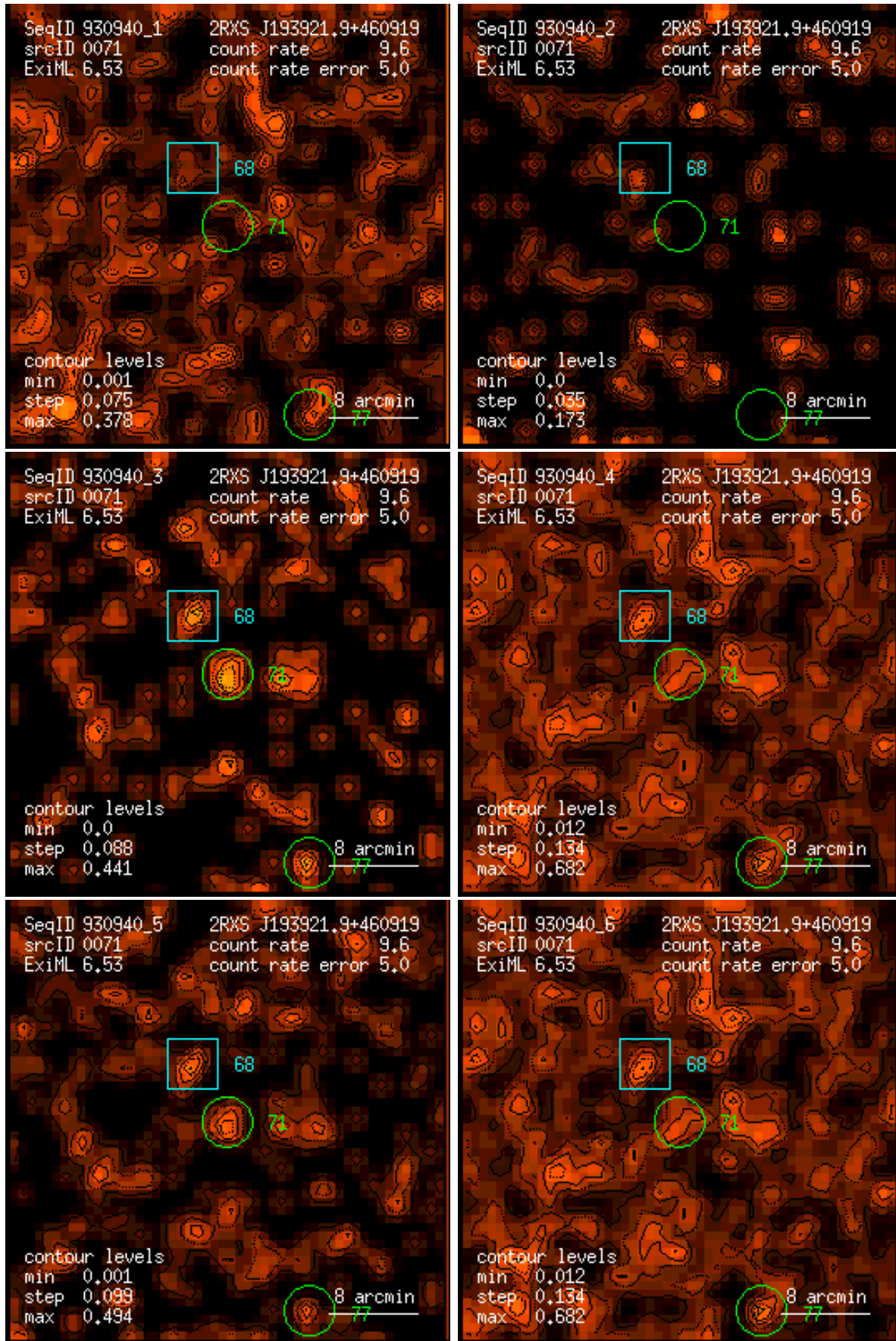
Figure 71: RASS 930940: detection 0071: band rate images, Gaussian filter: (1) PSPC channels 11 – 41, (2) 52 – 90, (3) 91 – 201, (4) 11 – 235, (5) 52 – 201, (6) 11 – 201. Broad band rates in counts/ks. Band rate contour levels in counts/ks/arcmin 2 .
