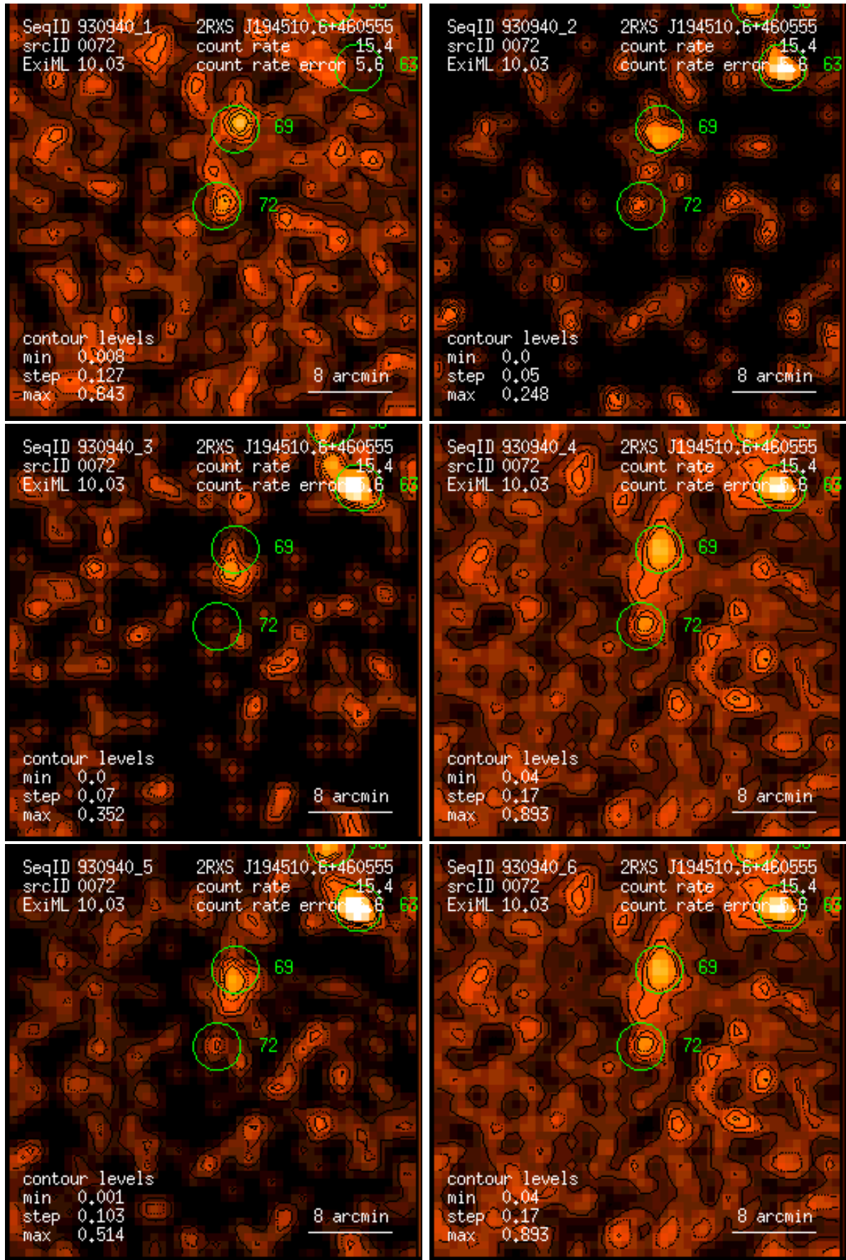
Figure 72: RASS 930940: detection 0072: band rate images, Gaussian filter: (1) PSPC channels 11 – 41, (2) 52 – 90, (3) 91 – 201, (4) 11 – 235, (5) 52 – 201, (6) 11 – 201. Broad band rates in counts/ks. Band rate contour levels in counts/ks/arcmin 2 .
