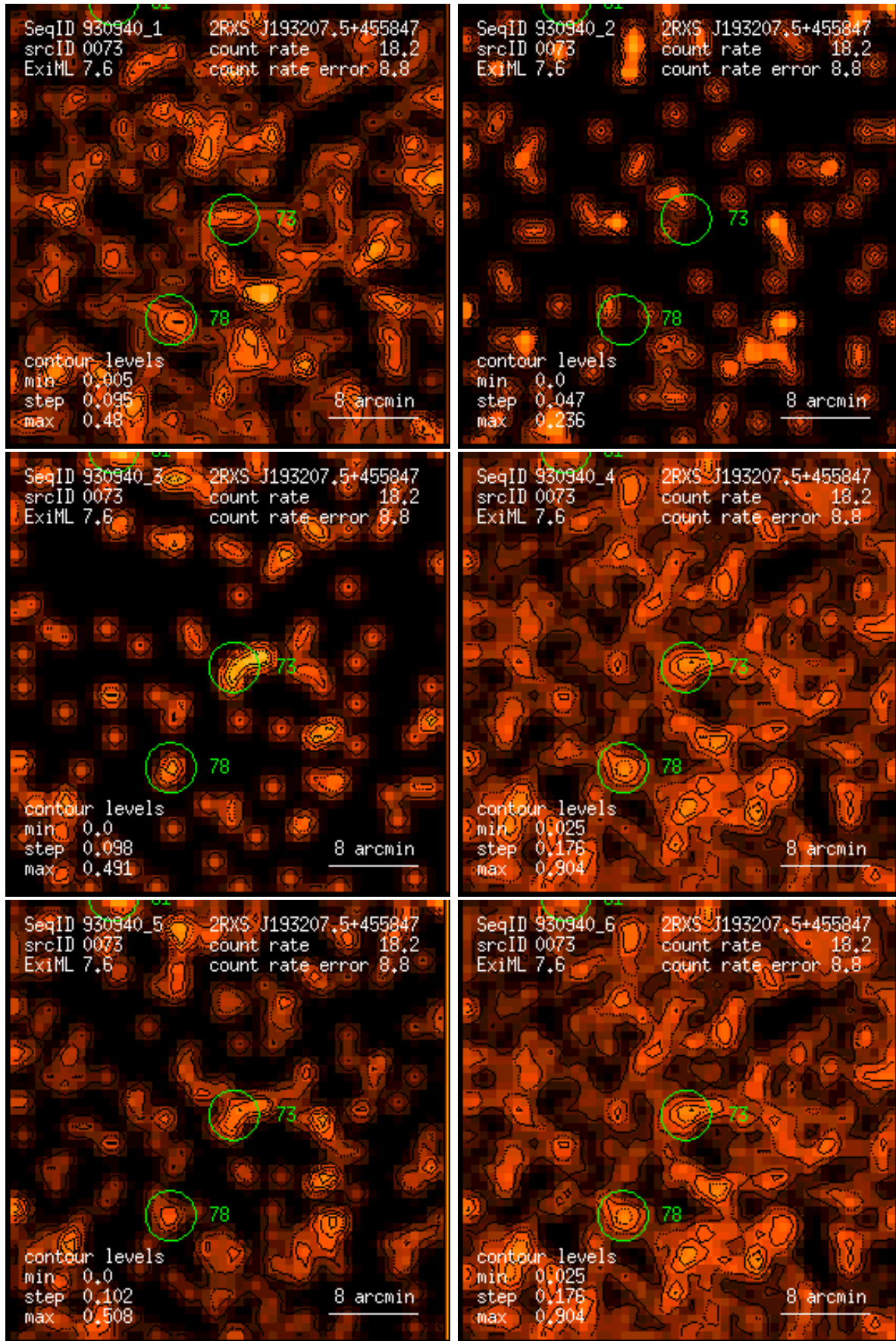
Figure 73: RASS 930940: detection 0073: band rate images, Gaussian filter: (1) PSPC channels 11 – 41, (2) 52 – 90, (3) 91 – 201, (4) 11 – 235, (5) 52 – 201, (6) 11 – 201. Broad band rates in counts/ks. Band rate contour levels in counts/ks/arcmin 2 .
