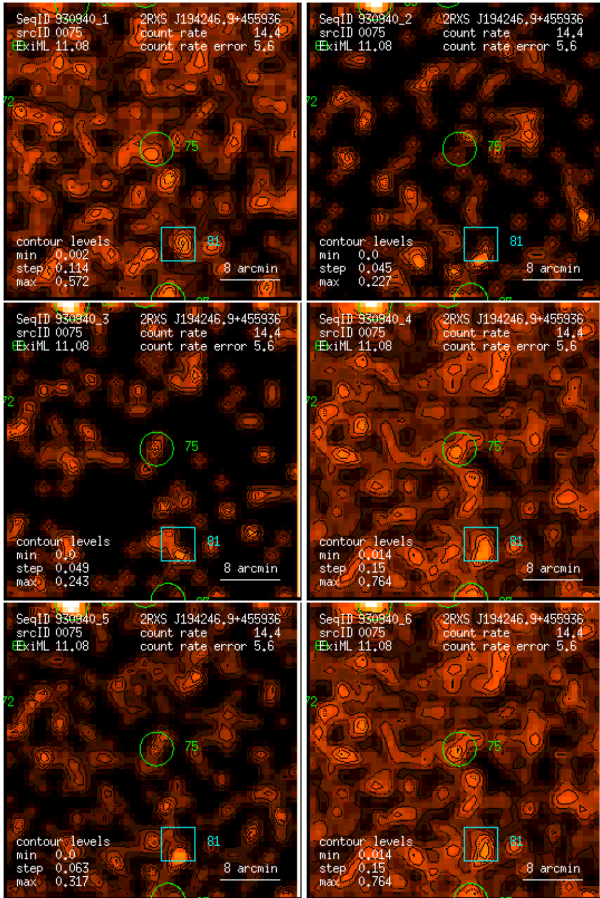
Figure 75: RASS 930940: detection 0075: band rate images, Gaussian filter: (1) PSPC channels 11 – 41, (2) 52 – 90, (3) 91 – 201, (4) 11 – 235, (5) 52 – 201, (6) 11 – 201. Broad band rates in counts/ks. Band rate contour levels in counts/ks/arcmin 2 .
