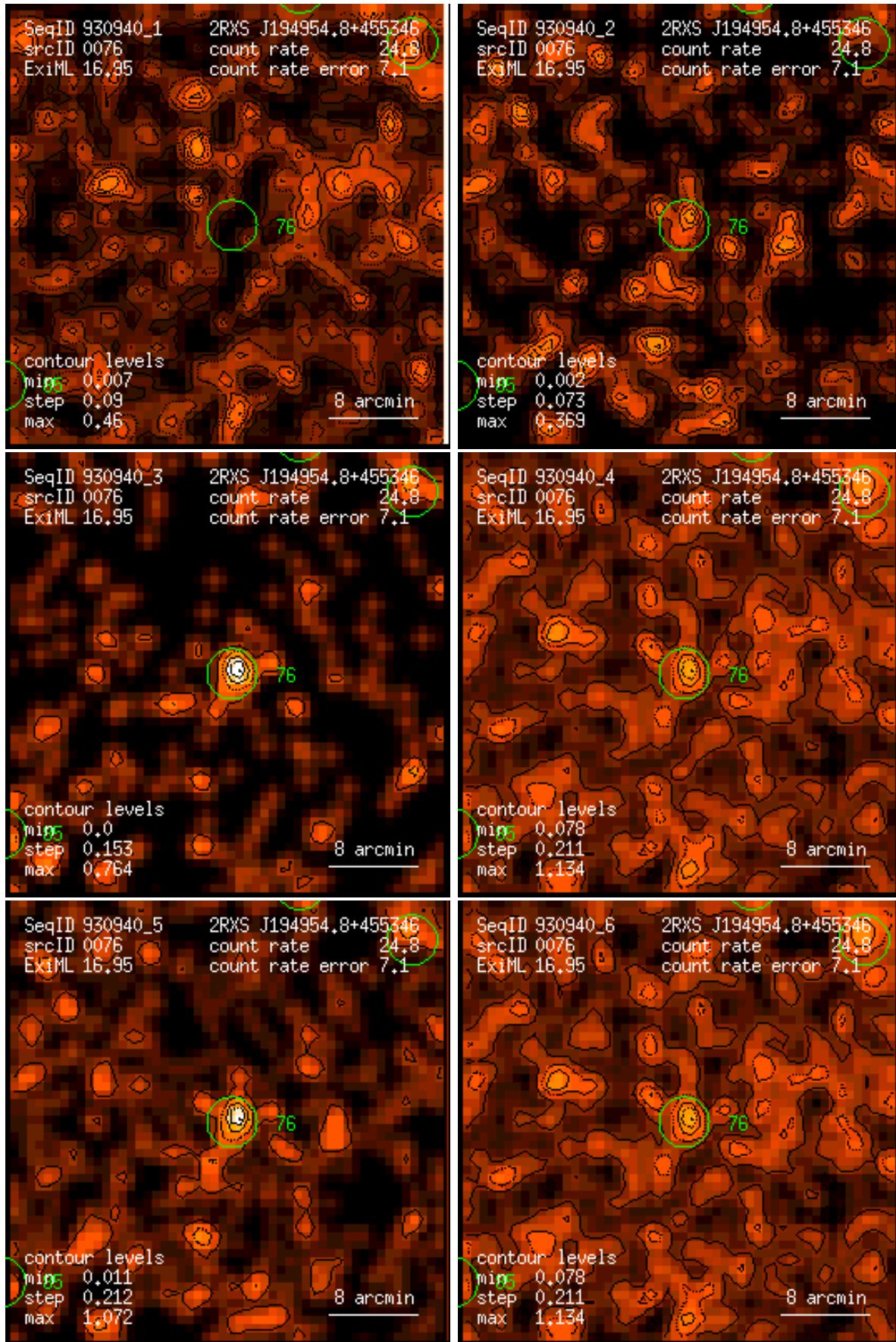
Figure 76: RASS 930940: detection 0076: band rate images, Gaussian filter: (1) PSPC channels 11 – 41, (2) 52 – 90, (3) 91 – 201, (4) 11 – 235, (5) 52 – 201, (6) 11 – 201. Broad band rates in counts/ks. Band rate contour levels in counts/ks/arcmin 2 .
