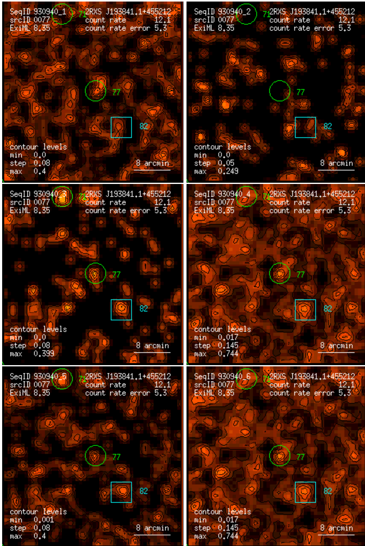
Figure 77: RASS 930940: detection 0077: band rate images, Gaussian filter: (1) PSPC channels 11 – 41, (2) 52 – 90, (3) 91 – 201, (4) 11 – 235, (5) 52 – 201, (6) 11 – 201. Broad band rates in counts/ks. Band rate contour levels in counts/ks/arcmin 2 .
