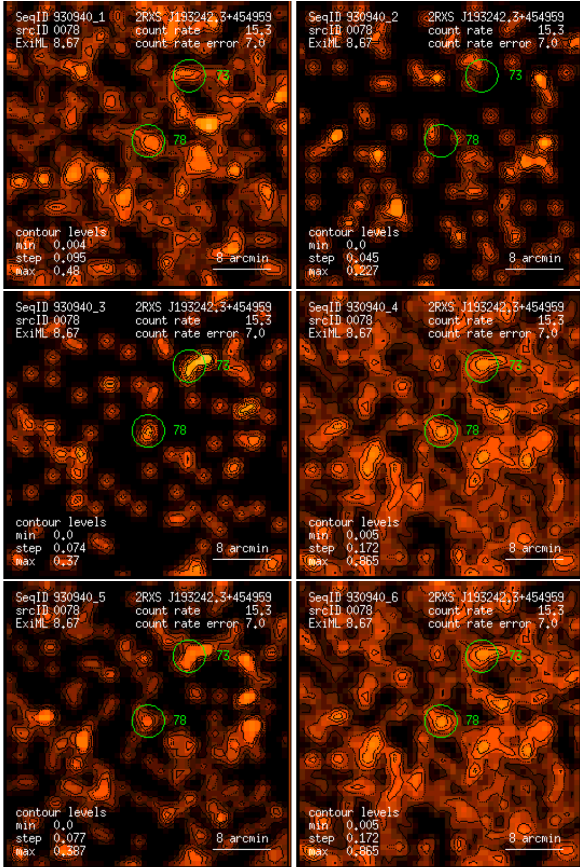
Figure 78: RASS 930940: detection 0078: band rate images, Gaussian filter: (1) PSPC channels 11 – 41, (2) 52 – 90, (3) 91 – 201, (4) 11 – 235, (5) 52 – 201, (6) 11 – 201. Broad band rates in counts/ks. Band rate contour levels in counts/ks/arcmin 2 .
