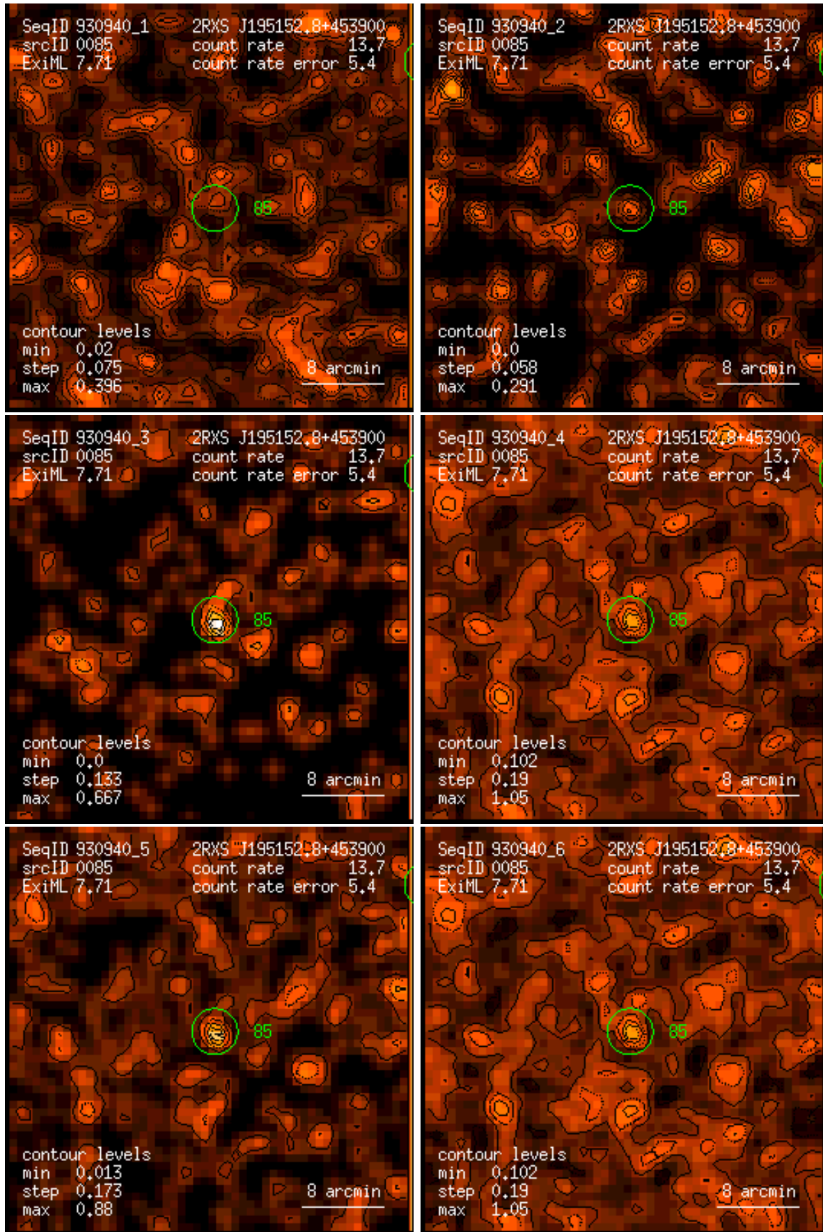
Figure 85: RASS 930940: detection 0085: band rate images, Gaussian filter: (1) PSPC channels 11 – 41, (2) 52 – 90, (3) 91 – 201, (4) 11 – 235, (5) 52 – 201, (6) 11 – 201. Broad band rates in counts/ks. Band rate contour levels in counts/ks/arcmin 2 .
