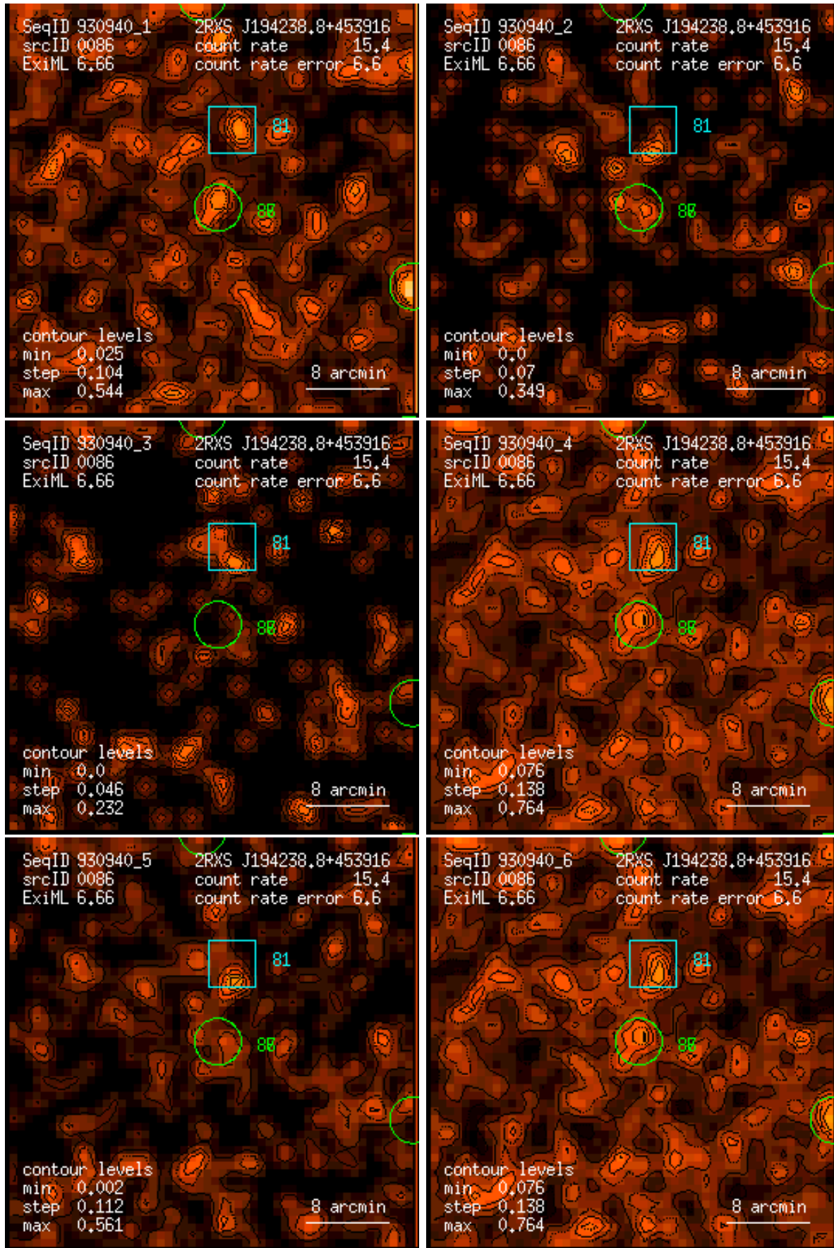
Figure 86: RASS 930940: detection 0086: band rate images, Gaussian filter: (1) PSPC channels 11 – 41, (2) 52 – 90, (3) 91 – 201, (4) 11 – 235, (5) 52 – 201, (6) 11 – 201. Broad band rates in counts/ks. Band rate contour levels in counts/ks/arcmin 2 .
