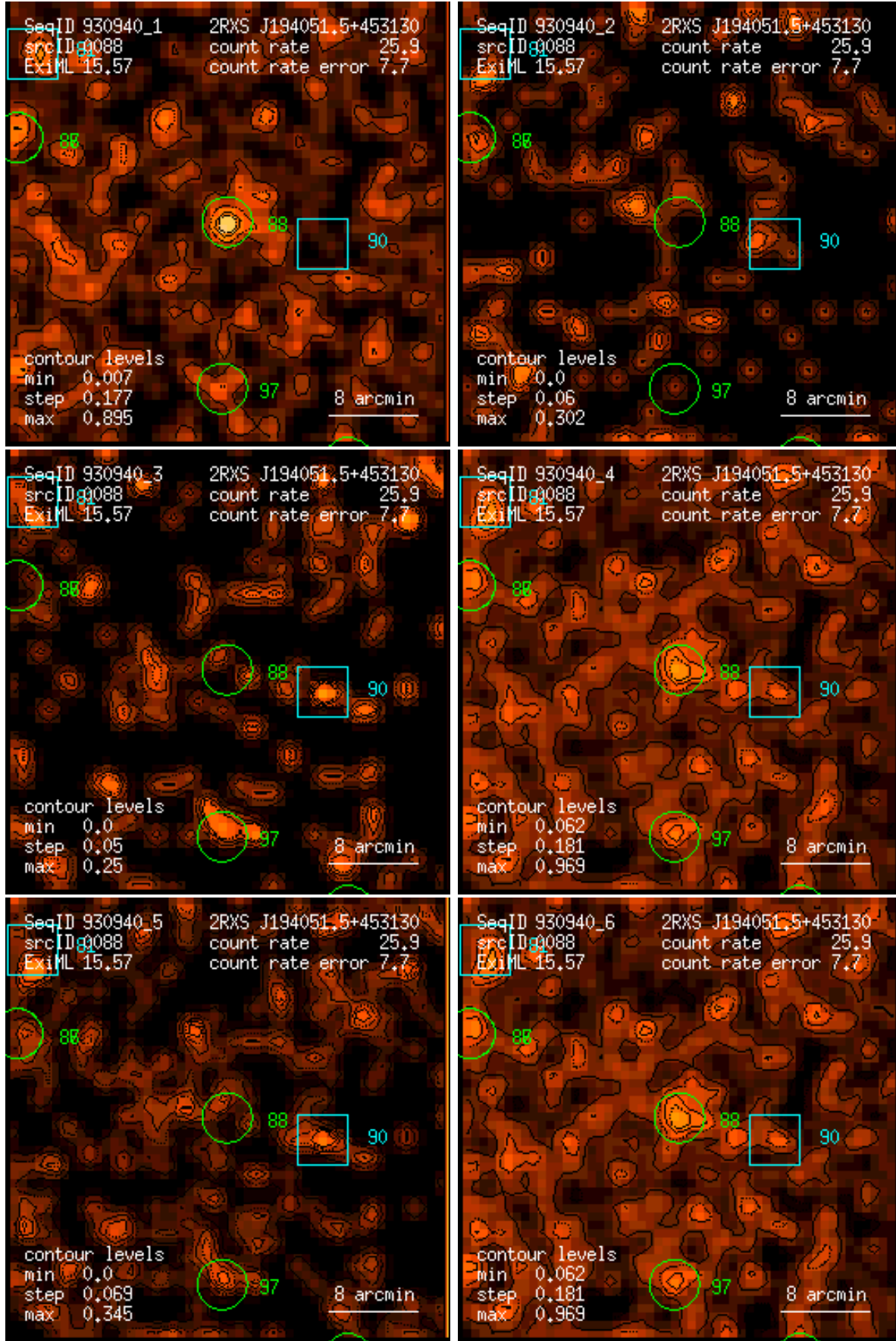
Figure 88: RASS 930940: detection 0088: band rate images, Gaussian filter: (1) PSPC channels 11 – 41, (2) 52 – 90, (3) 91 – 201, (4) 11 – 235, (5) 52 – 201, (6) 11 – 201. Broad band rates in counts/ks. Band rate contour levels in counts/ks/arcmin 2 .
