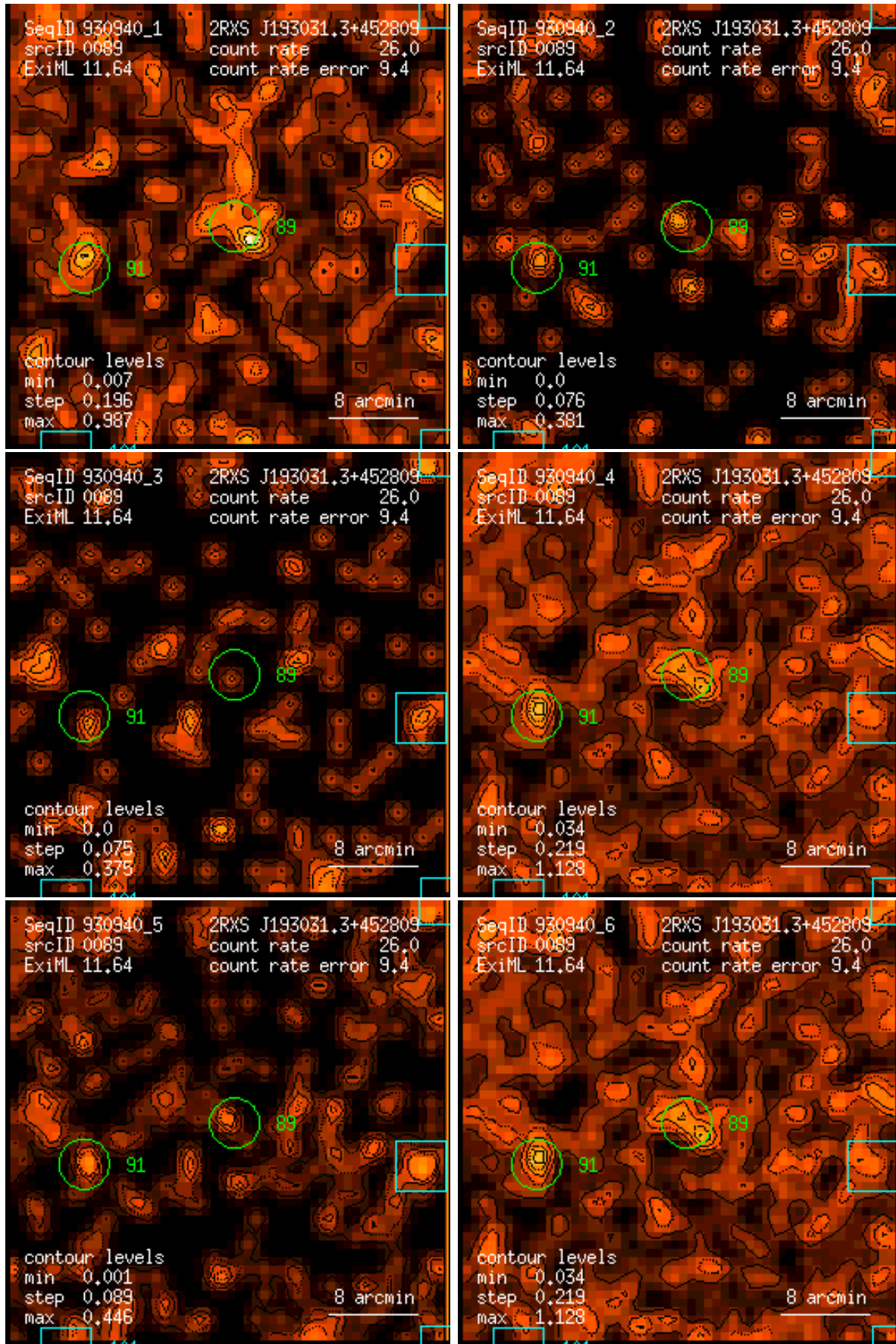
Figure 89: RASS 930940: detection 0089: band rate images, Gaussian filter: (1) PSPC channels 11 – 41, (2) 52 – 90, (3) 91 – 201, (4) 11 – 235, (5) 52 – 201, (6) 11 – 201. Broad band rates in counts/ks. Band rate contour levels in counts/ks/arcmin 2 .
