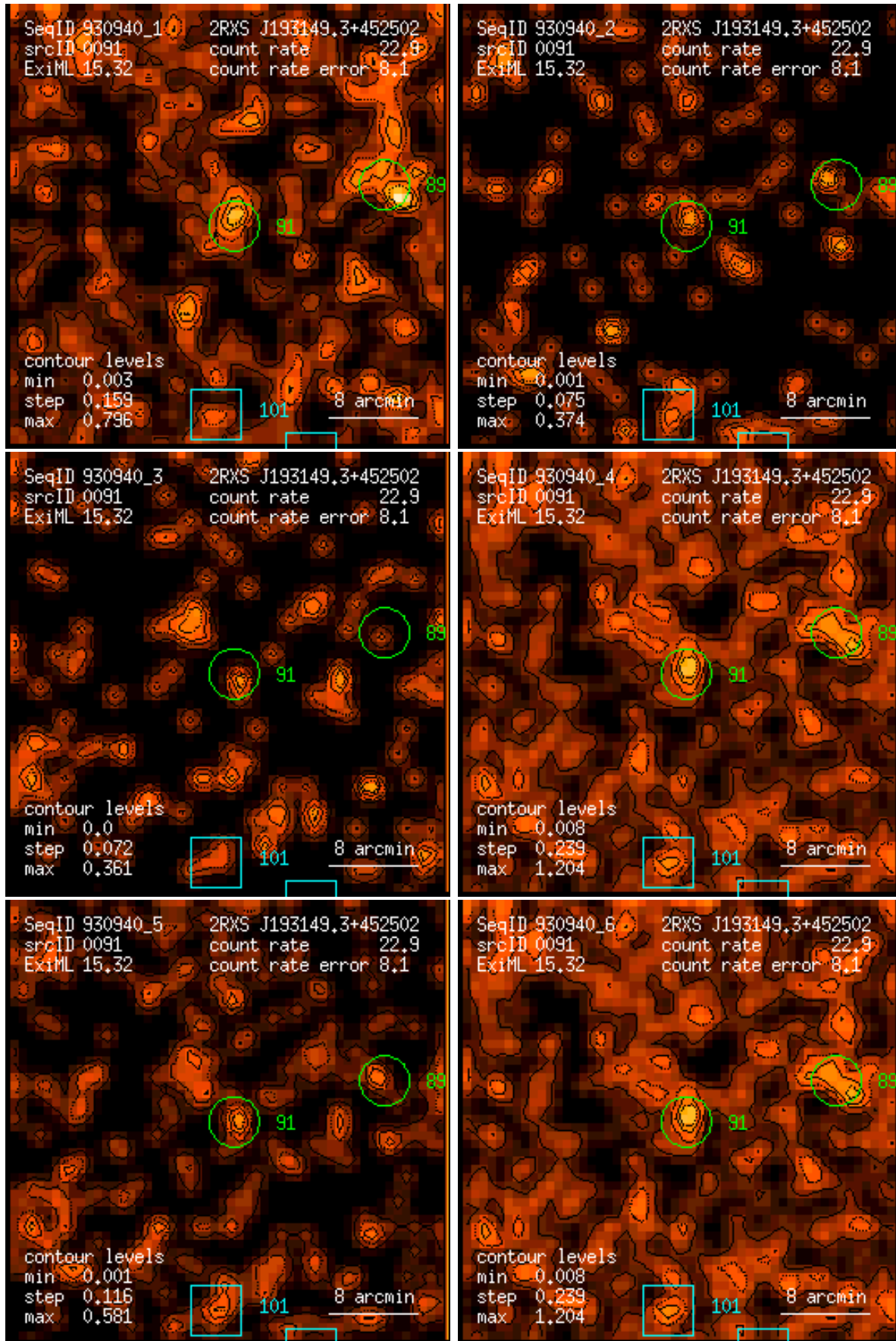
Figure 91: RASS 930940: detection 0091: band rate images, Gaussian filter: (1) PSPC channels 11 – 41, (2) 52 – 90, (3) 91 – 201, (4) 11 – 235, (5) 52 – 201, (6) 11 – 201. Broad band rates in counts/ks. Band rate contour levels in counts/ks/arcmin 2 .
