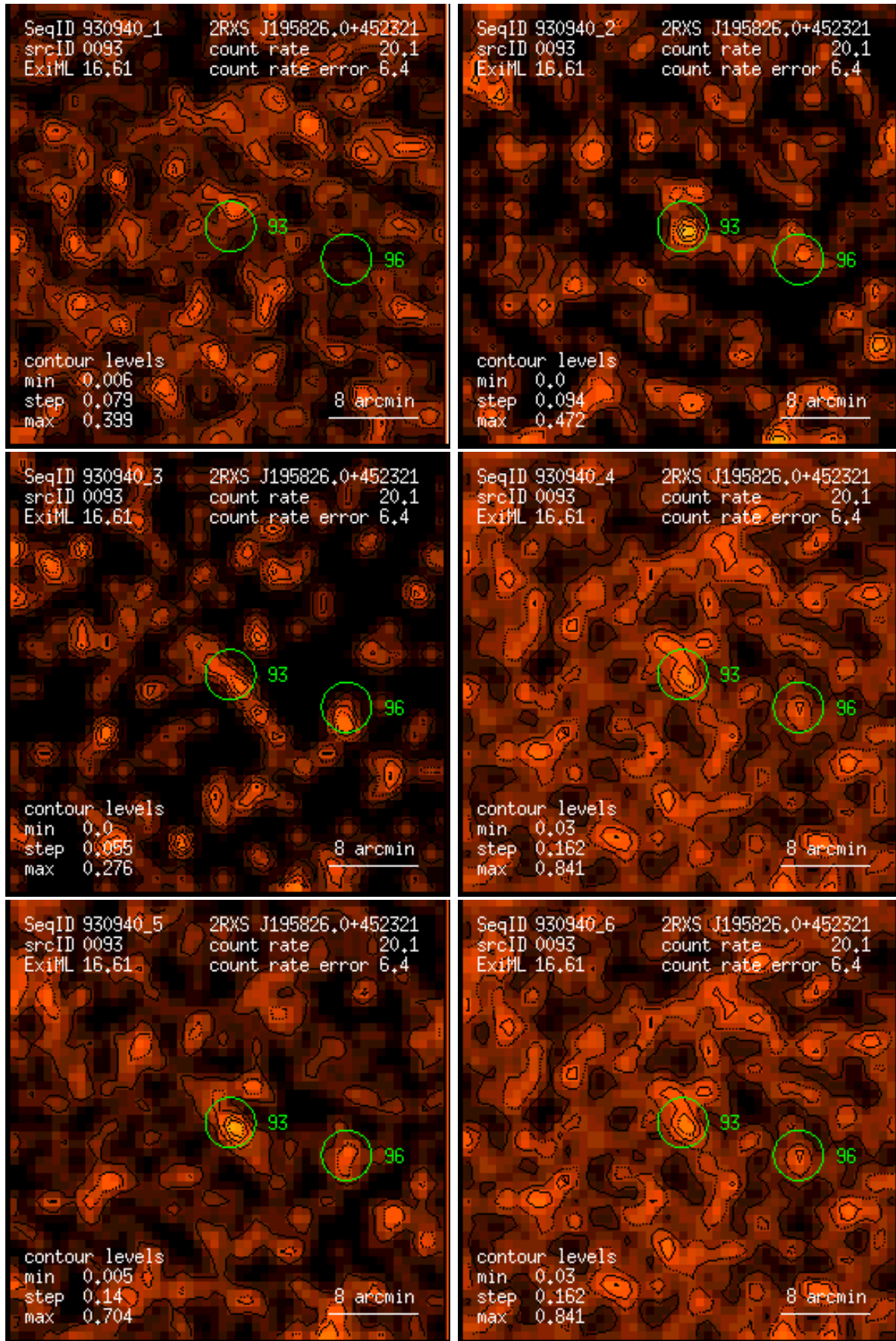
Figure 93: RASS 930940: detection 0093: band rate images, Gaussian filter: (1) PSPC channels 11 – 41, (2) 52 – 90, (3) 91 – 201, (4) 11 – 235, (5) 52 – 201, (6) 11 – 201. Broad band rates in counts/ks. Band rate contour levels in counts/ks/arcmin 2 .
