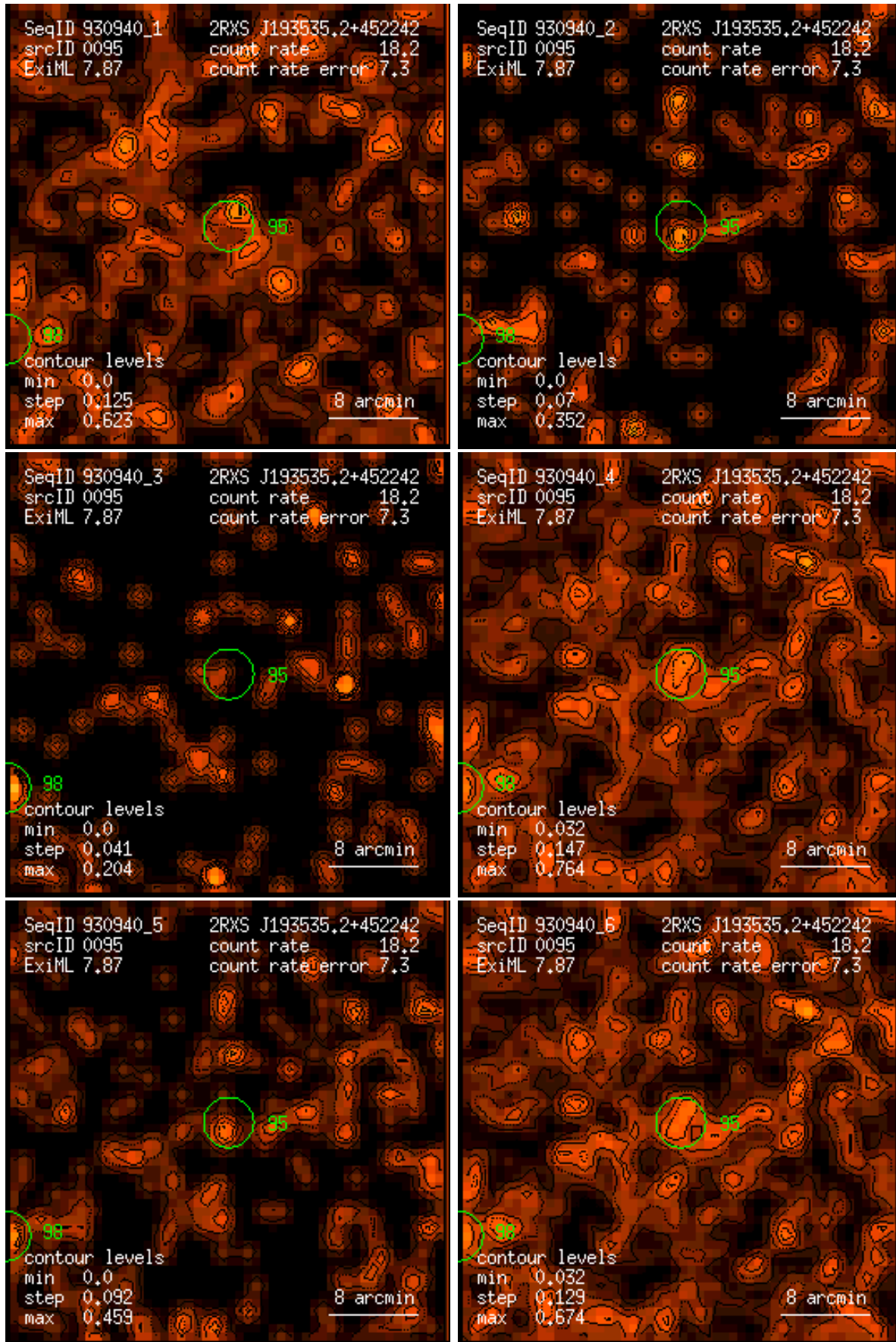
Figure 95: RASS 930940: detection 0095: band rate images, Gaussian filter: (1) PSPC channels 11 – 41, (2) 52 – 90, (3) 91 – 201, (4) 11 – 235, (5) 52 – 201, (6) 11 – 201. Broad band rates in counts/ks. Band rate contour levels in counts/ks/arcmin 2 .
