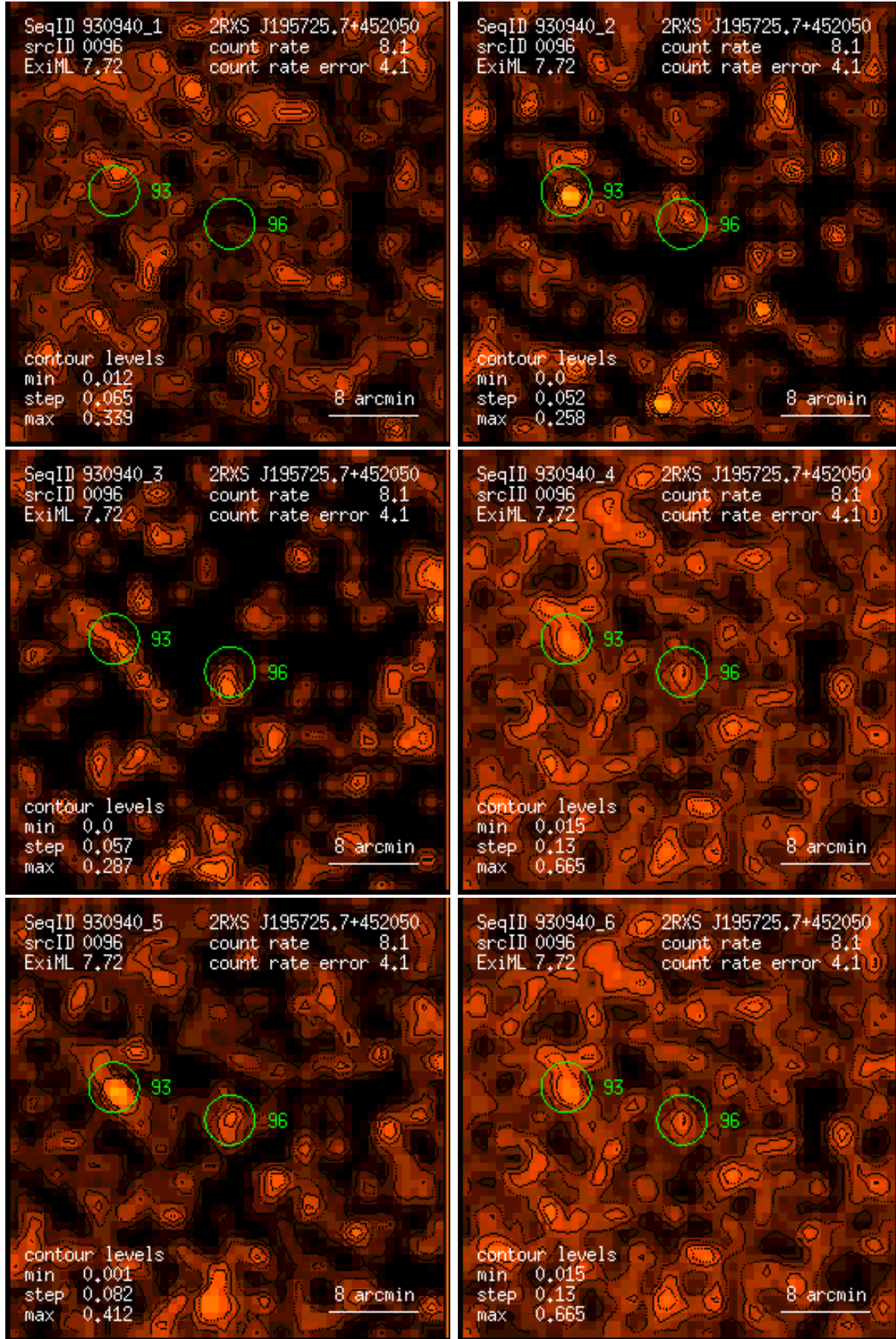
Figure 96: RASS 930940: detection 0096: band rate images, Gaussian filter: (1) PSPC channels 11 – 41, (2) 52 – 90, (3) 91 – 201, (4) 11 – 235, (5) 52 – 201, (6) 11 – 201. Broad band rates in counts/ks. Band rate contour levels in counts/ks/arcmin 2 .
