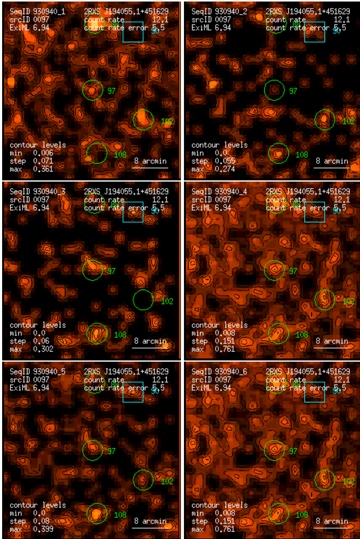
Figure 97: RASS 930940: detection 0097: band rate images, Gaussian filter: (1) PSPC channels 11 – 41, (2) 52 – 90, (3) 91 – 201, (4) 11 – 235, (5) 52 – 201, (6) 11 – 201. Broad band rates in counts/ks. Band rate contour levels in counts/ks/arcmin 2 .
